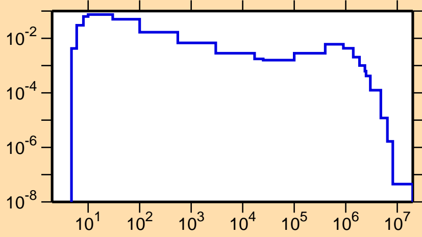
\sigma vs. E for ^{148}\text{Ho}(n,n_3)
