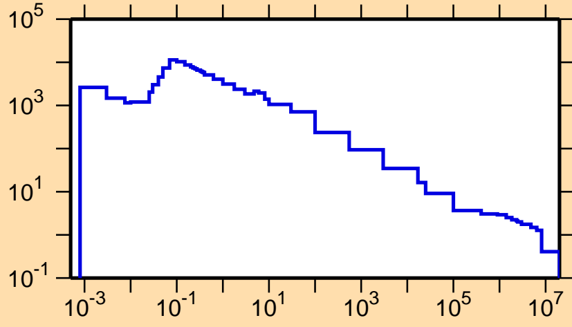
\sigma vs. E for ^{148}\text{Ho}(n,p)
