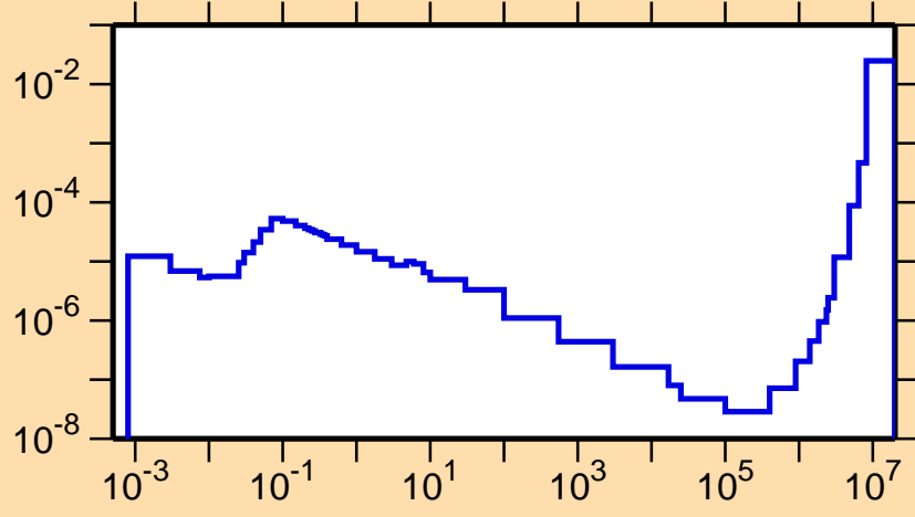
\sigma vs. E for ^{148}\text{Ho}(n,p\alpha)
