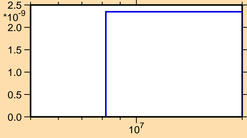
\sigma vs. E for ^{148}\text{Ho}(\text{mt117})
