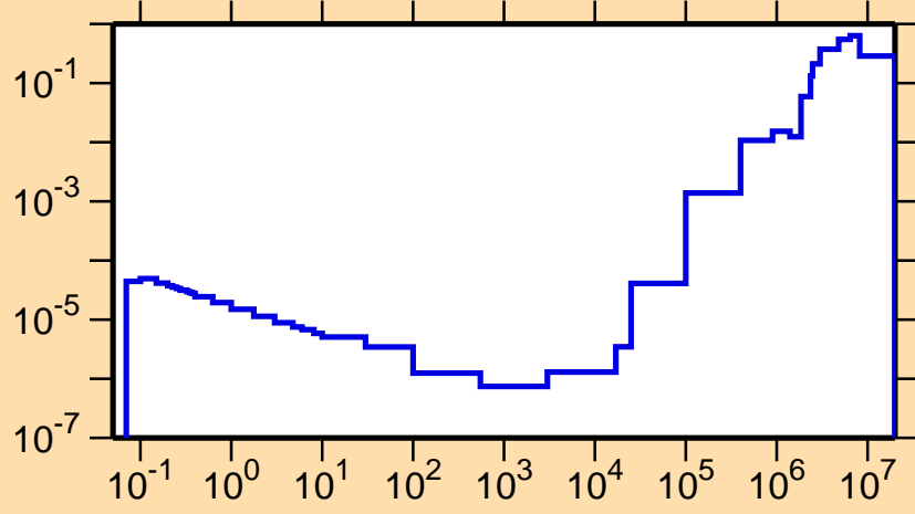
\sigma vs. E for ^{148}\text{Ho}(n,n\text{cont.})
