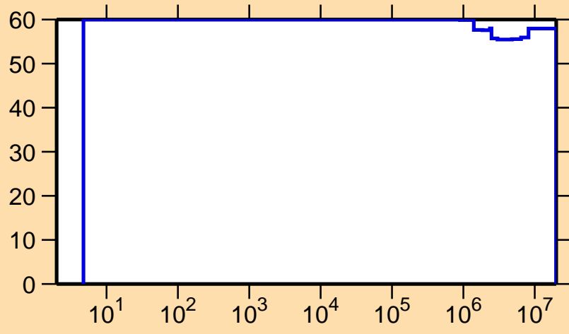
\Delta\sigma/\sigma vs. E for ^{148}\text{Ho}(n,n_1)
