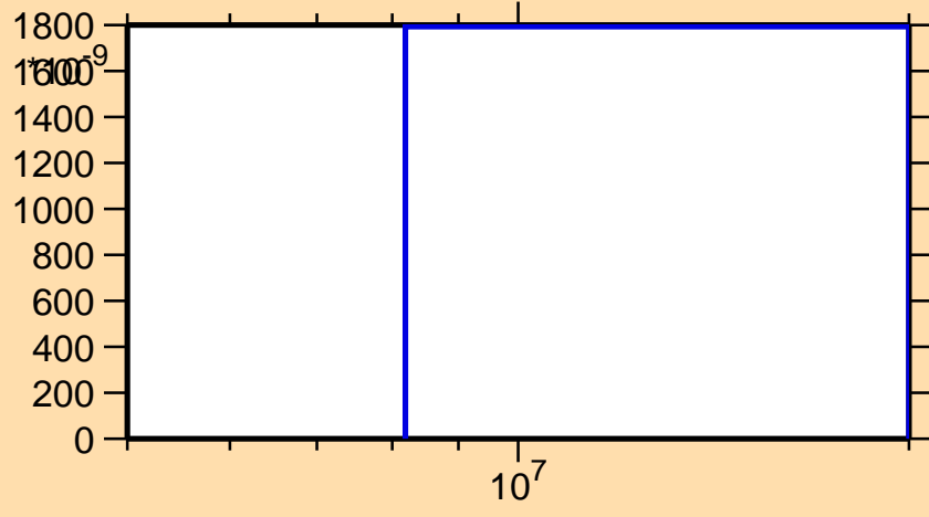
\sigma vs. E for ^{148}\text{Ho} (mt 45)
