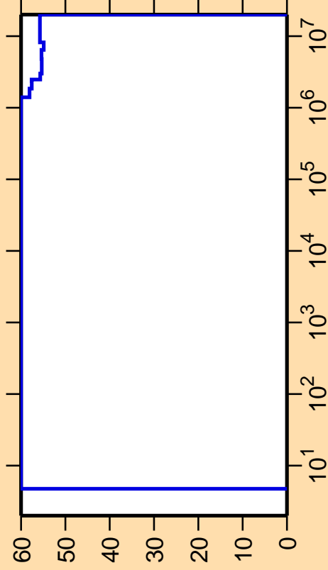
\Delta\sigma/\sigma vs. E for ^{148}\text{Ho}(n,n_3)
