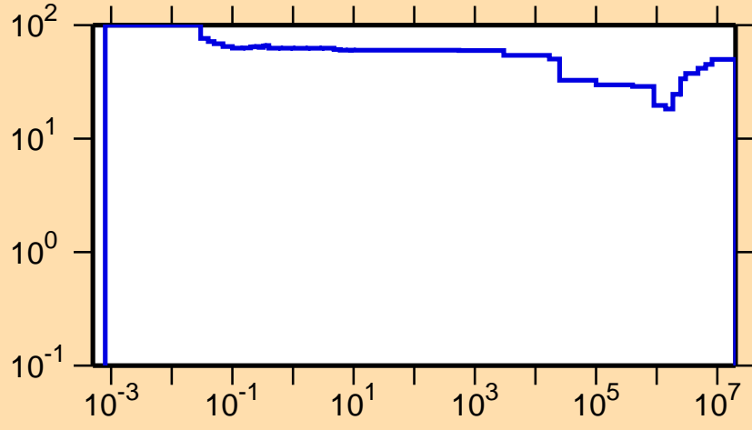
\Delta\sigma/\sigma vs. E for ^{148}\text{Ho}(n,p)
