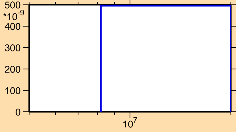
\sigma vs. E for ^{148}\text{Ho}(n,\text{nd})
