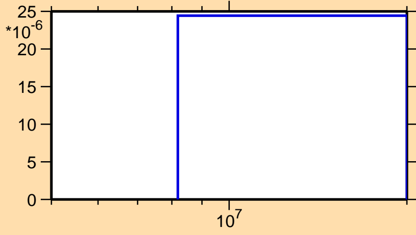
\sigma vs. E for ^{148}\text{Ho}(n,\text{pd})
