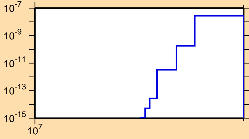
\sigma vs. E for ^{149}\text{Ho}(n,\text{pt})
