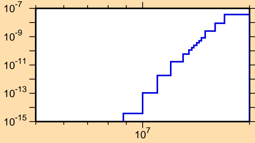
\sigma vs. E for ^{149}\text{Ho}(\text{mt117})
