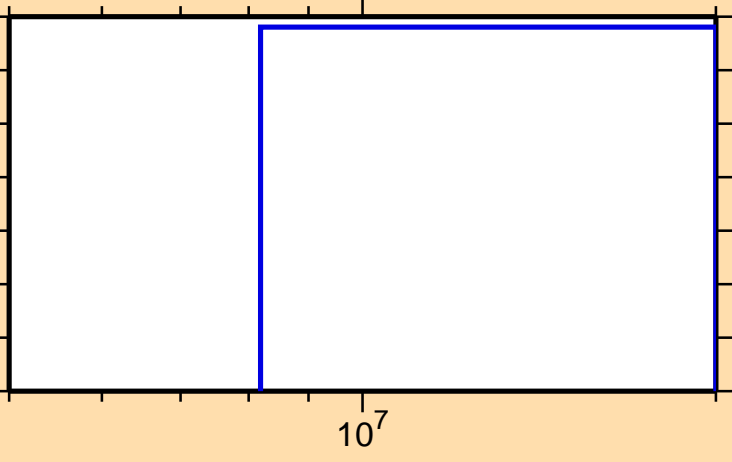
\sigma vs. E for ^{149}\text{Ho}(\text{mt } 45)
