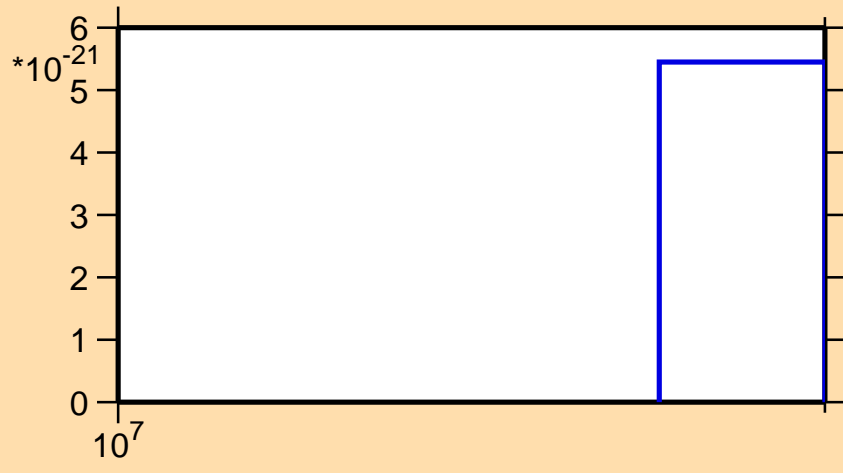
\sigma vs. E for ^{150}\text{Ho} (mt 11)
