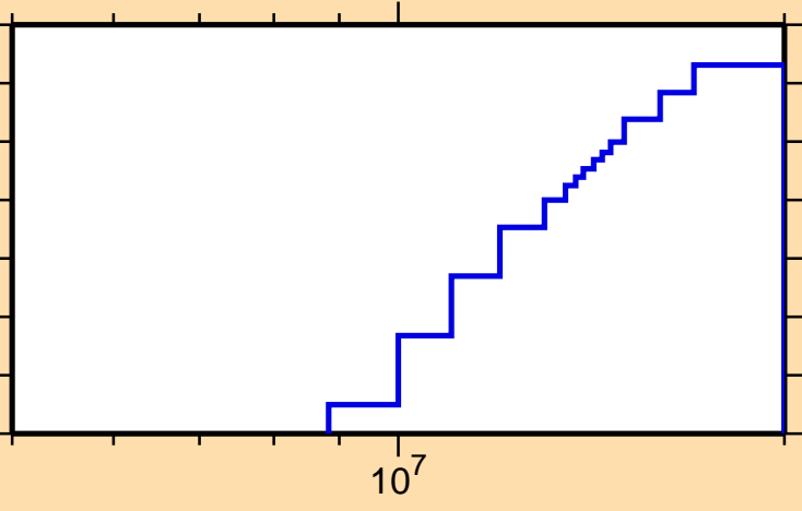
\sigma vs. E for ^{150}\text{Ho}(\text{mt117})
