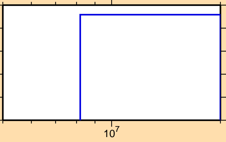
\sigma vs. E for ^{150}\text{Ho}(\text{mt117})
