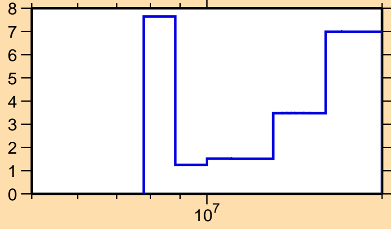
\Delta\sigma/\sigma vs. E for ^{150}\text{Ho}(n,\text{tot.})
