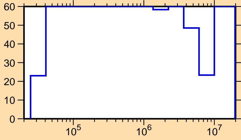
\Delta\sigma/\sigma vs. E for ^{150}\text{Ho}(n,n_1)
