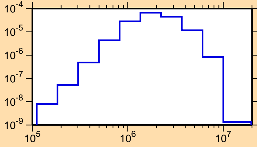
\sigma vs. E for ^{150}\text{Ho}(n,n_1)
