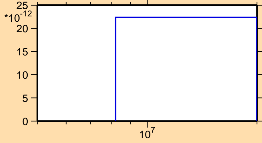
\sigma vs. E for ^{150}\text{Ho}(n,nt)
