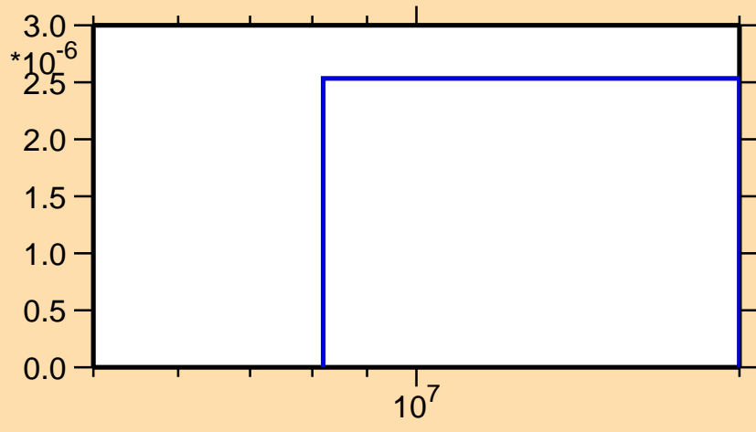
\sigma vs. E for ^{150}\text{Ho}(n,\text{nd})
