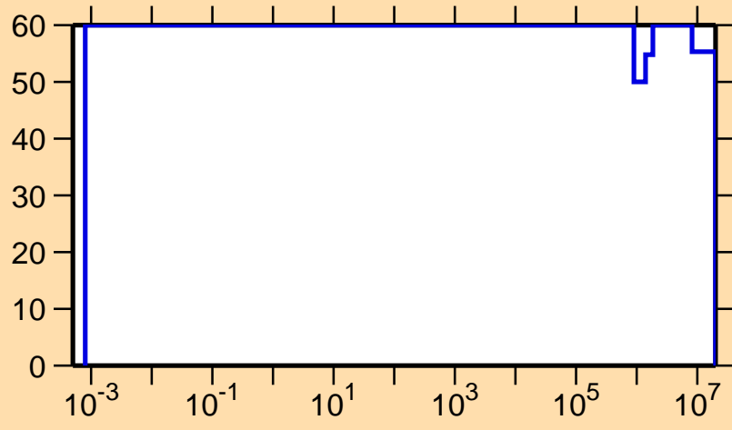
\Delta\sigma/\sigma vs. E for ^{150}\text{Ho}(n,p)
