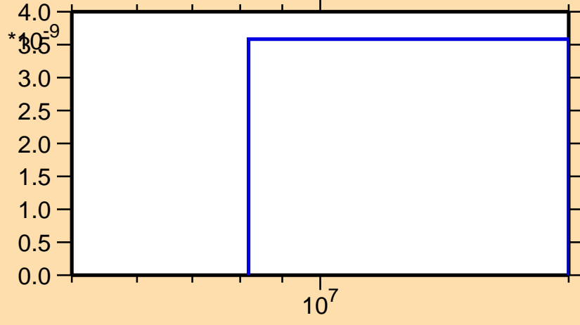
\sigma vs. E for ^{150}\text{Ho}(\text{mt117})
