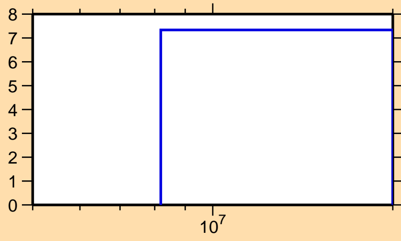
\Delta\sigma/\sigma vs. E for ^{150}\text{Ho}(n,\text{el.})
