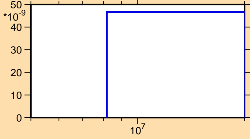
\sigma vs. E for ^{150}\text{Ho}(n,\text{pt})
