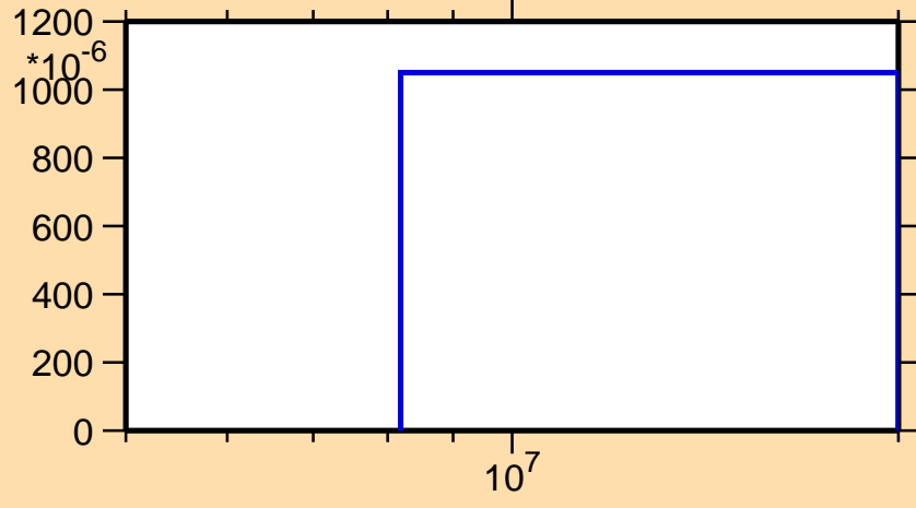
\sigma vs. E for ^{150}\text{Ho}(n,2np)
