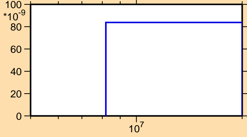
\sigma vs. E for ^{150}\text{Ho}(n,2n\alpha)
