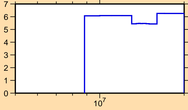
\Delta\sigma/\sigma vs. E for ^{151}\text{Ho}(n,\text{nonel.})
