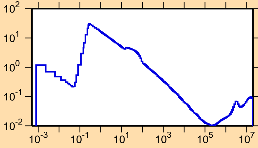
\sigma vs. E for ^{151}\text{Ho}(n,\alpha)
