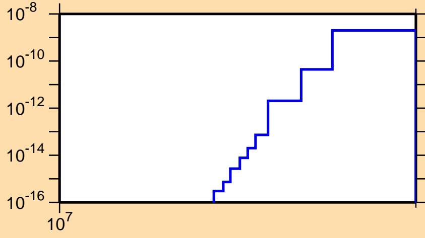
\sigma vs. E for ^{151}\text{Ho} (mt 34)
