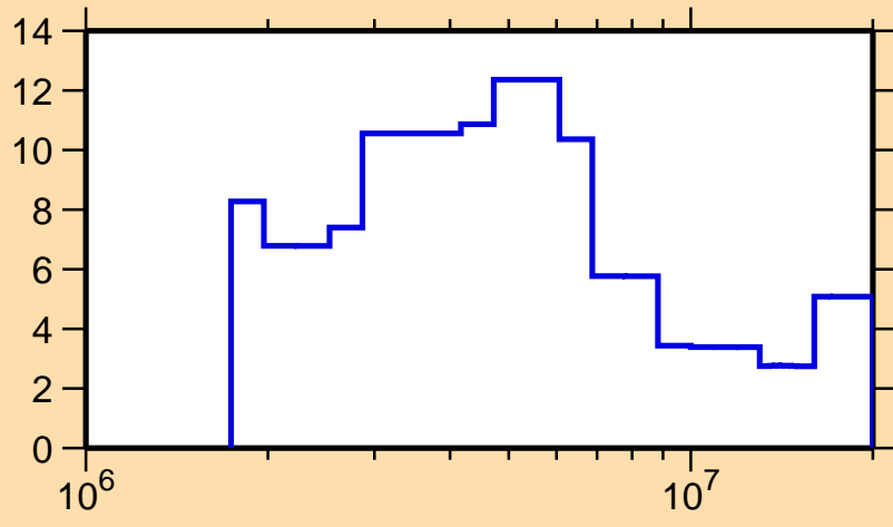
\Delta\sigma/\sigma vs. E for ^{151}\text{Ho}(n,\text{tot.})
