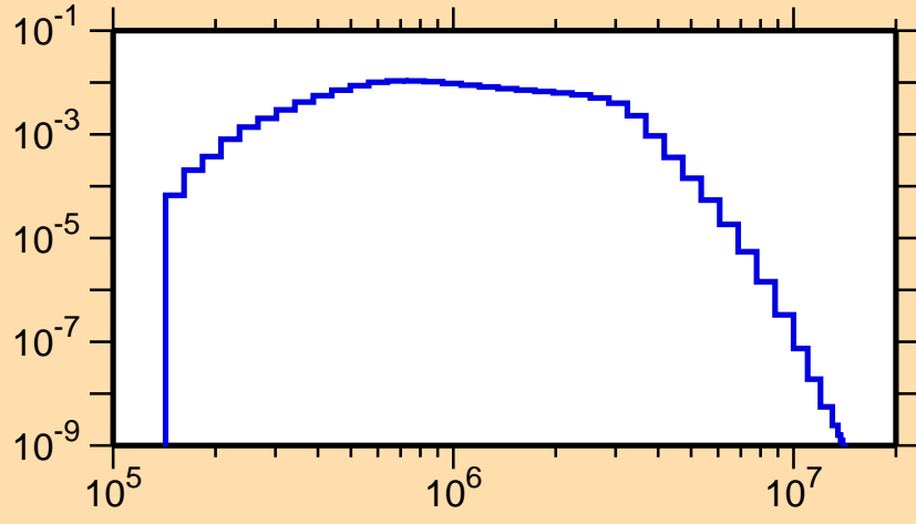
\sigma vs. E for ^{151}\text{Ho}(n,n_2)
