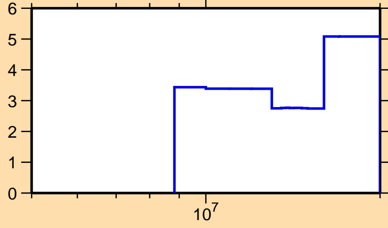
\Delta\sigma/\sigma vs. E for ^{151}\text{Ho}(n,\text{tot.})
