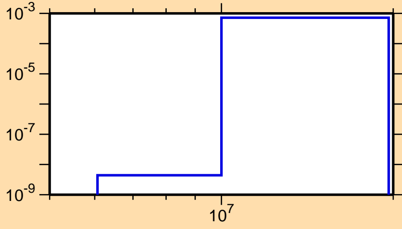
\sigma vs. E for ^{151}\text{Ho}(n,t)
