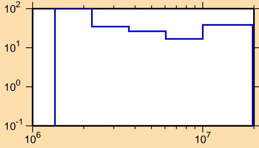
\Delta\sigma/\sigma vs. E for ^{151}\text{Ho}(n,n\text{cont.})
