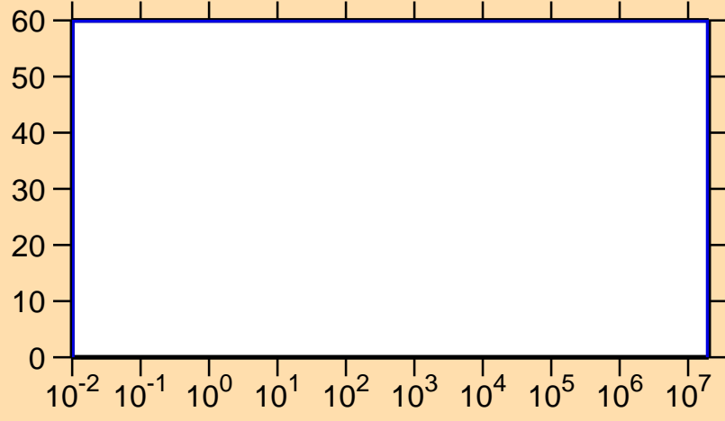
\Delta\sigma/\sigma vs. E for ^{151}\text{Ho}(n,p)
