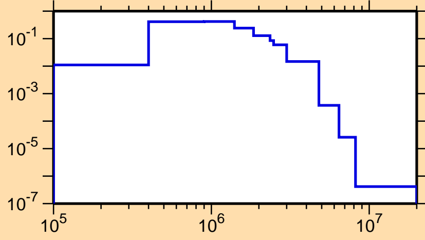
\sigma vs. E for ^{151}\text{Ho}(n,n_3)
