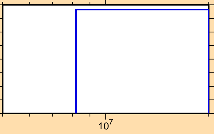
\sigma vs. E for ^{151}\text{Ho}(n,nt)
