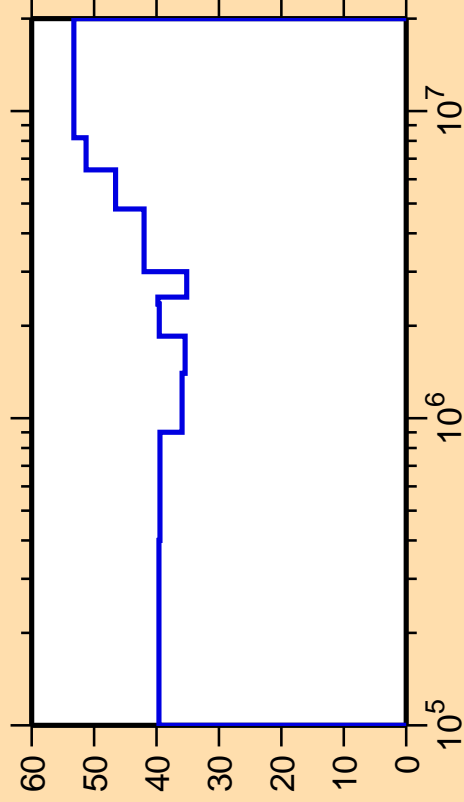
\Delta\sigma/\sigma vs. E for ^{151}\text{Ho}(n,n_2)
