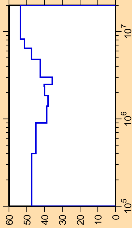
\Delta\sigma/\sigma vs. E for ^{151}\text{Ho}(n,n_3)
