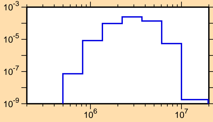
\sigma vs. E for ^{152}\text{Ho}(n,n_4)
