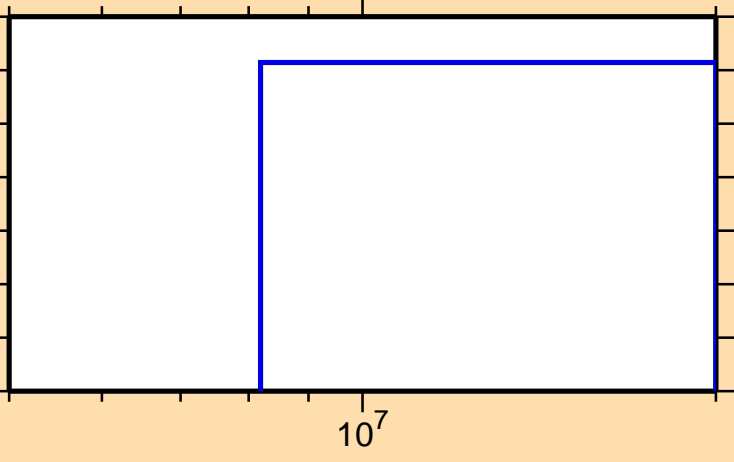
\sigma vs. E for ^{152}\text{Ho}(n,nt)
