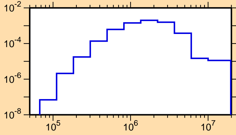
\sigma vs. E for ^{153}\text{Ho}(n,n_1)
