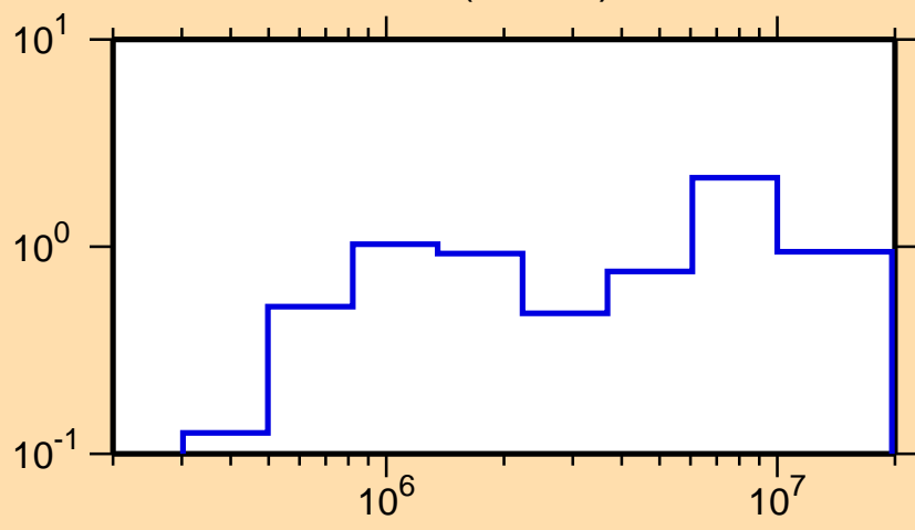
\sigma vs. E for ^{153}\text{Ho}(n,\text{inel.})
