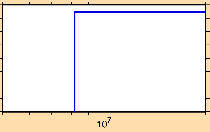
\sigma vs. E for ^{153}\text{Ho}(n,\text{nd})
