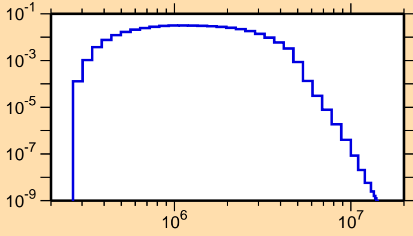
\sigma vs. E for ^{153}\text{Ho}(n,n_3)
