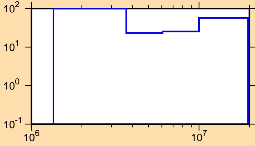
\Delta\sigma/\sigma vs. E for ^{153}\text{Ho}(n,n\text{cont.})
