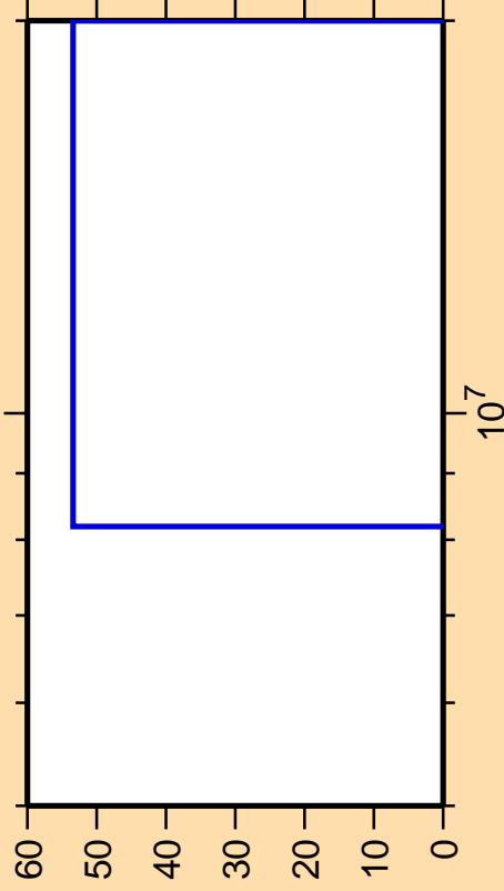
\Delta\sigma/\sigma vs. E for ^{154}\text{Ho}(n,3n)
