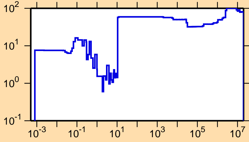
\Delta\sigma/\sigma vs. E for ^{154}\text{Ho}(n,\gamma)
