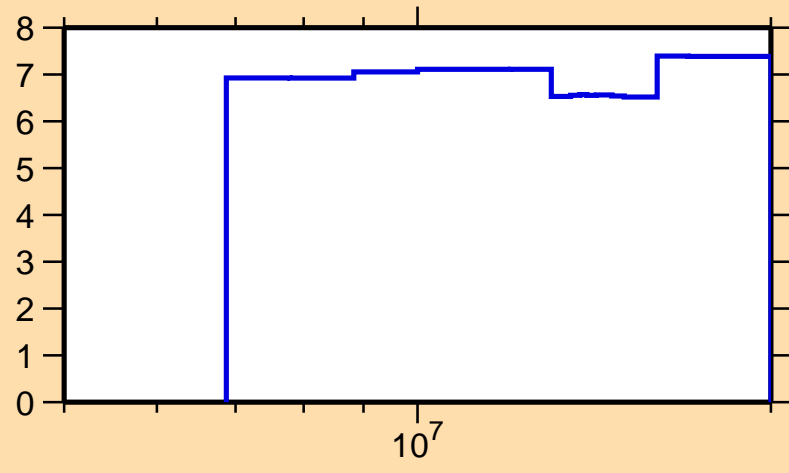
\Delta\sigma/\sigma vs. E for ^{154}\text{Ho}(n,\text{nonel.})
