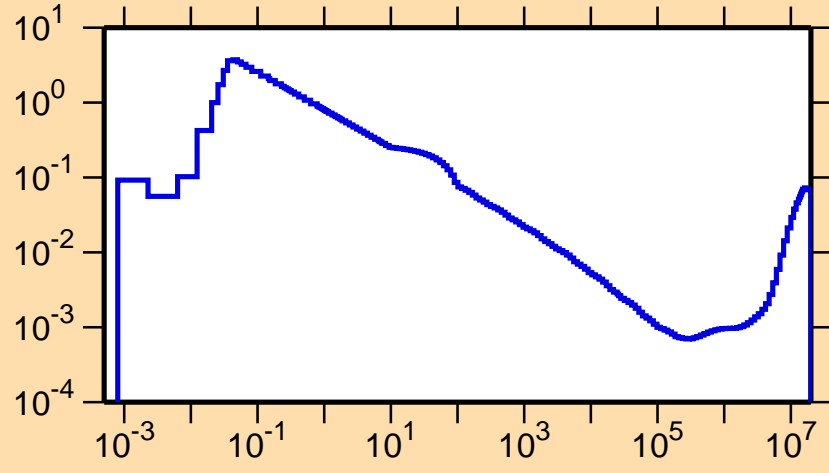
\sigma vs. E for ^{154}\text{Ho}(n,\alpha)
