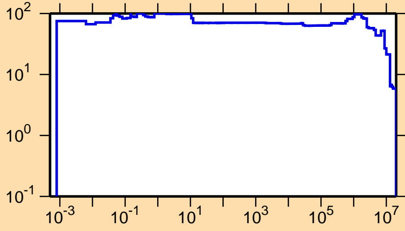
\Delta\sigma/\sigma vs. E for ^{154}\text{Ho}(n,p)
