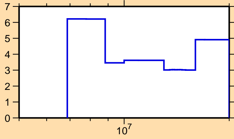
\Delta\sigma/\sigma vs. E for ^{154}\text{Ho}(n,\text{tot.})
