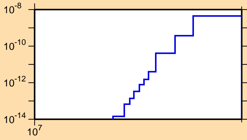
\sigma vs. E for ^{154}\text{Ho}(n,\text{pd})
