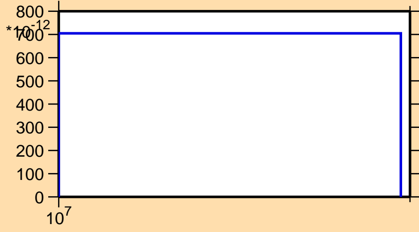
\sigma vs. E for ^{154}\text{Ho}(n,3n\alpha)
