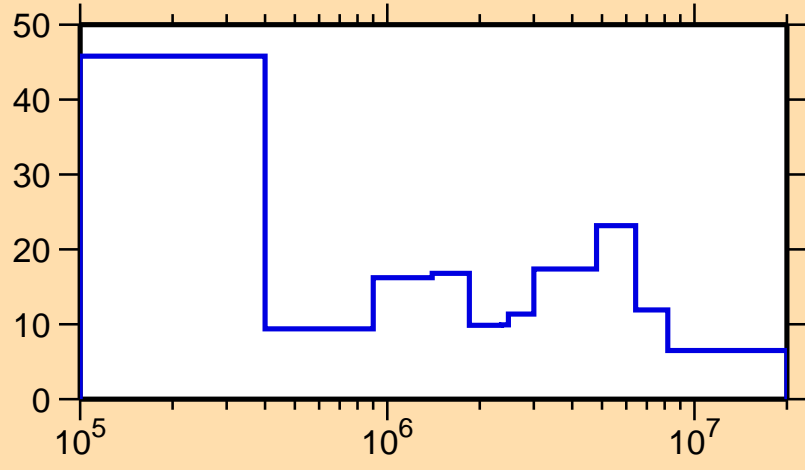
\Delta\sigma/\sigma vs. E for ^{154}\text{Ho}(n, el.)
