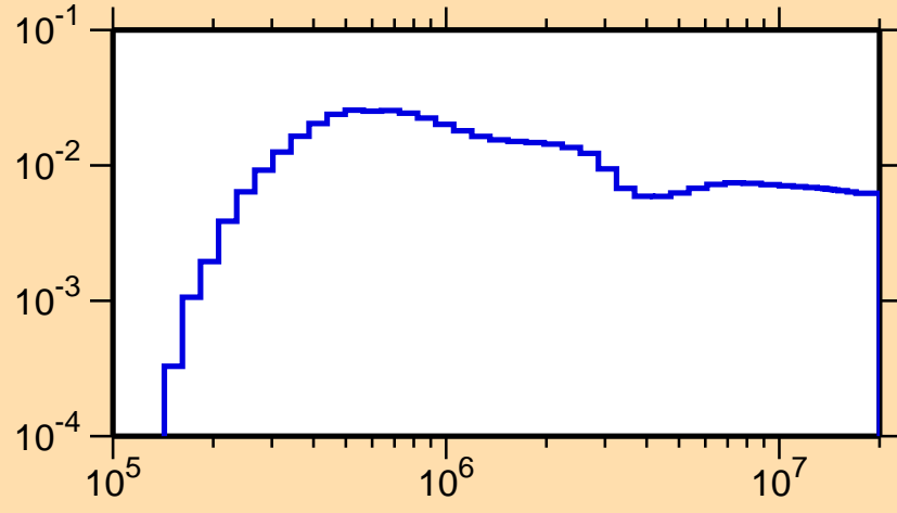
\sigma vs. E for ^{155}\text{Ho}(n,n_2)
