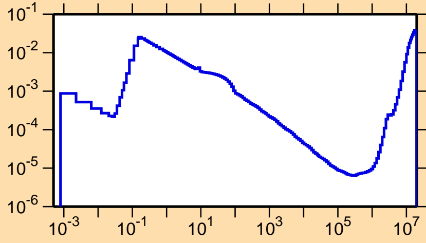
\sigma vs. E for ^{155}\text{Ho}(n,\alpha)
