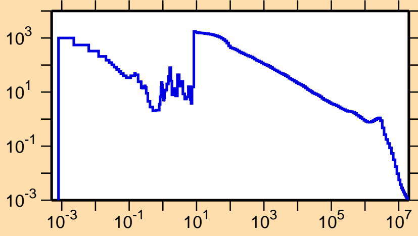
\sigma vs. E for ^{155}\text{Ho}(n,\gamma)
