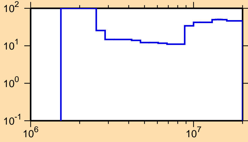
\Delta\sigma/\sigma vs. E for ^{155}\text{Ho}(n,n\text{cont.})
