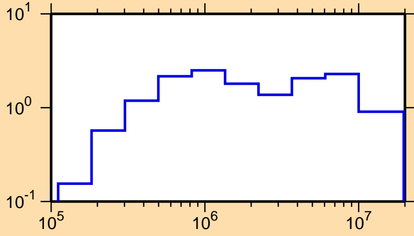
\sigma vs. E for ^{155}\text{Ho}(n,\text{inel.})
