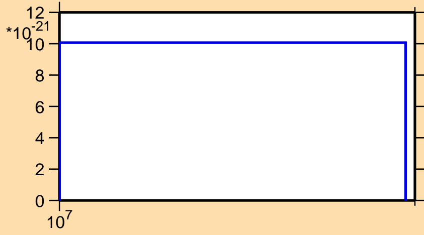
\sigma vs. E for ^{155}\text{Ho} (mt 42)
