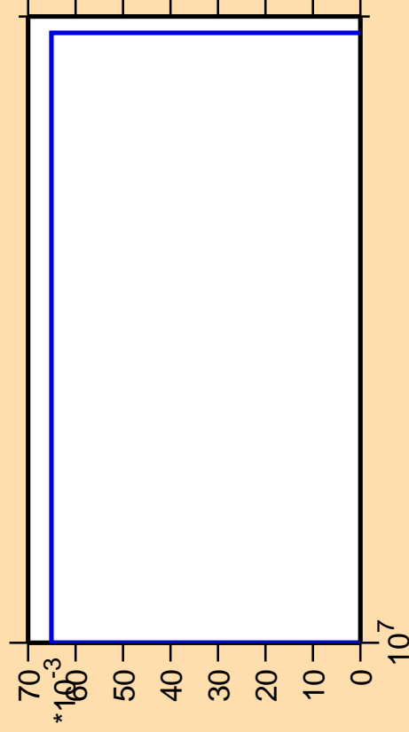
\Delta\sigma/\sigma vs. E for ^{155}\text{Ho} (mt 34)
