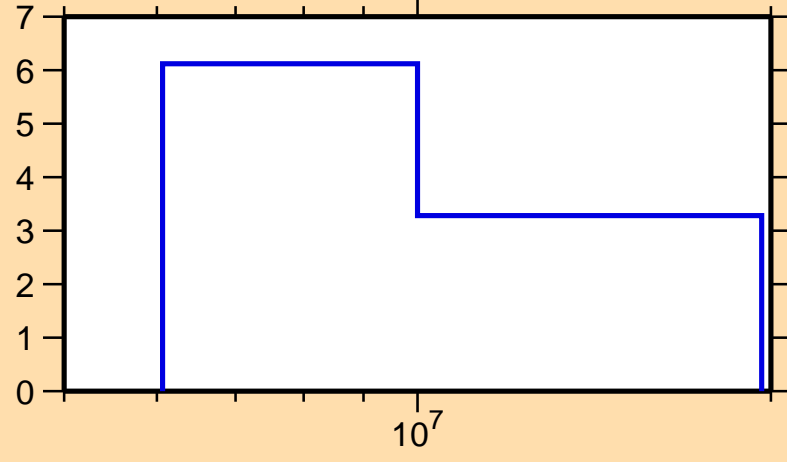
\Delta\sigma/\sigma vs. E for ^{155}\text{Ho}(n,\text{tot.})
