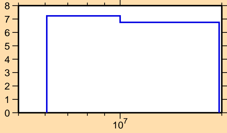
\Delta\sigma/\sigma vs. E for ^{155}\text{Ho}(n,\text{el.})
