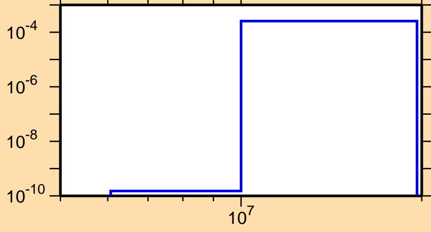
\sigma vs. E for ^{155}\text{Ho}(n,t)
