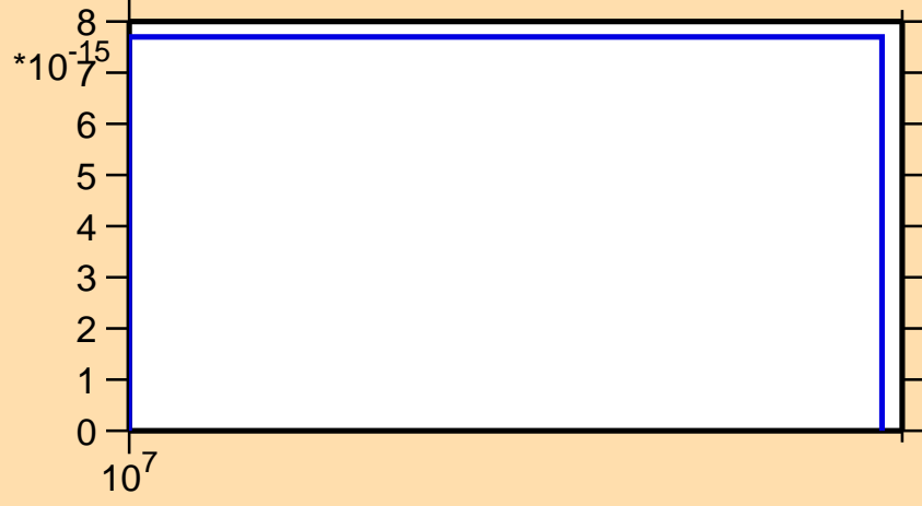
\sigma vs. E for ^{155}\text{Ho} (mt 34)
