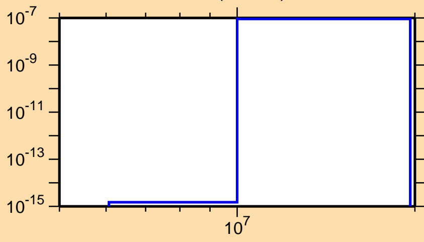
\sigma vs. E for ^{155}\text{Ho}(n,\text{He3})
