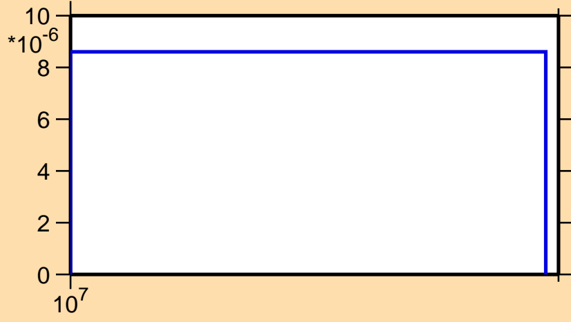
\sigma vs. E for ^{155}\text{Ho}(n,2np)
