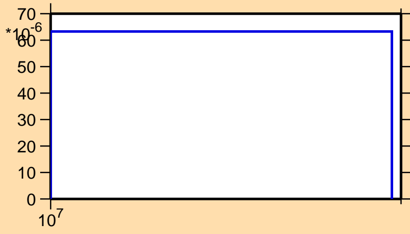
\sigma vs. E for ^{155}\text{Ho}(n,3n)
