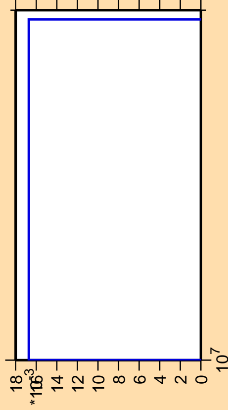
\Delta\sigma/\sigma vs. E for ^{155}\text{Ho}(n,\text{pt})
