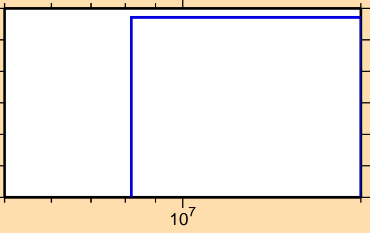
\sigma vs. E for ^{155}\text{Ho}(n,3n)
