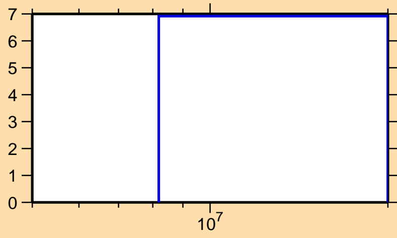
\Delta\sigma/\sigma vs. E for ^{155}\text{Ho}(n,\text{nonel.})
