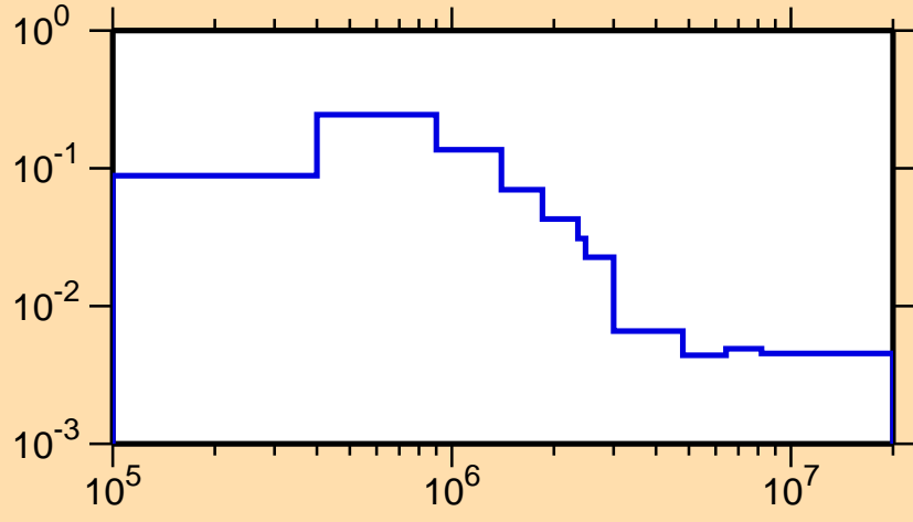
\sigma vs. E for ^{155}\text{Ho}(n,n_3)
