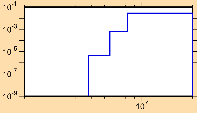
\sigma vs. E for ^{155}\text{Ho}(n,np)
