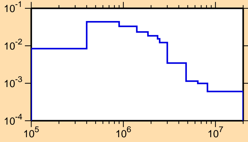
\sigma vs. E for ^{155}\text{Ho}(n,n_4)
