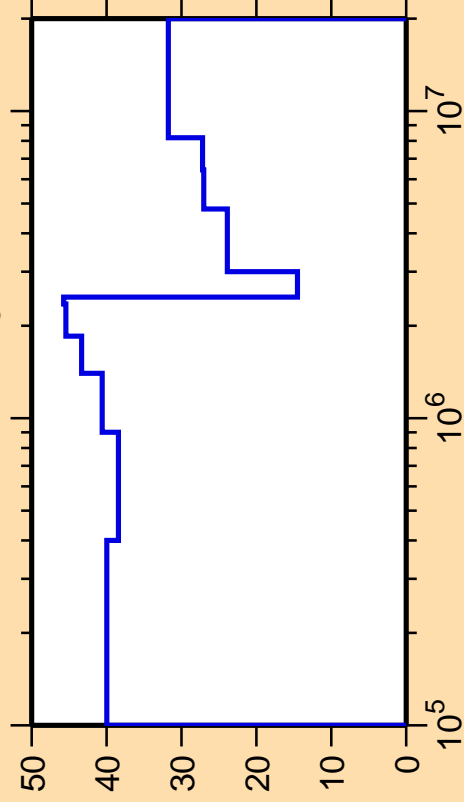
\Delta\sigma/\sigma vs. E for ^{155}\text{Ho}(n,n_3)
