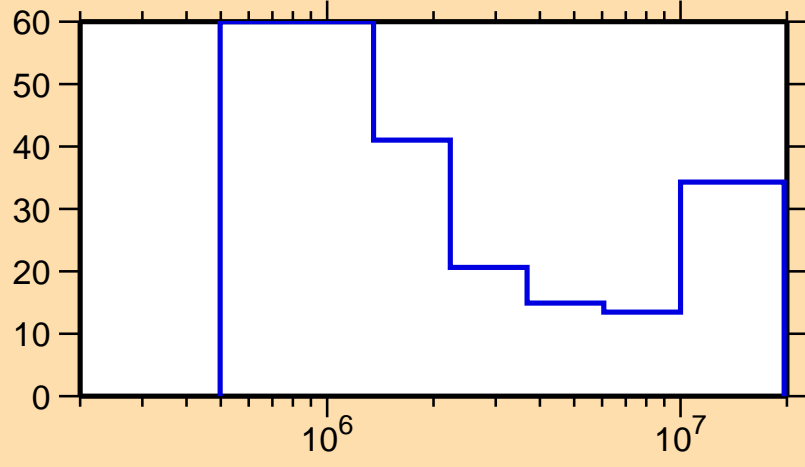
\Delta\sigma/\sigma vs. E for ^{156}\text{Ho}(n,n\text{cont.})
