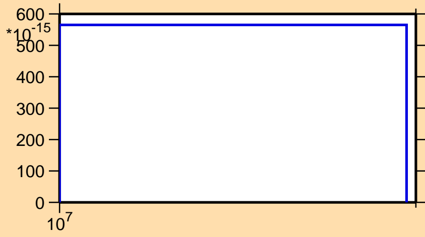
\sigma vs. E for ^{156}\text{Ho} (mt 34)
