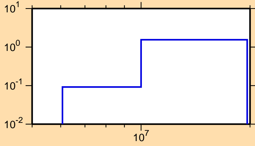
\sigma vs. E for ^{156}\text{Ho}(n,2n)
