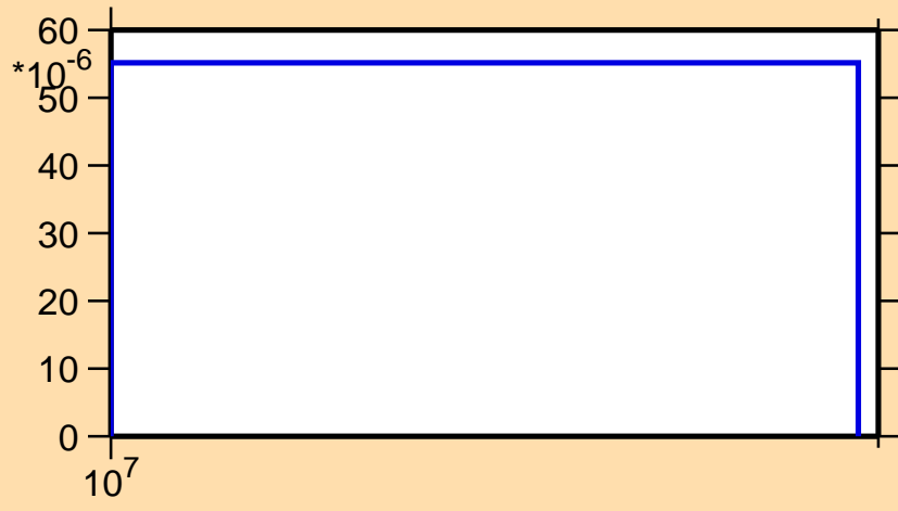
\sigma vs. E for ^{156}\text{Ho}(n,3n)
