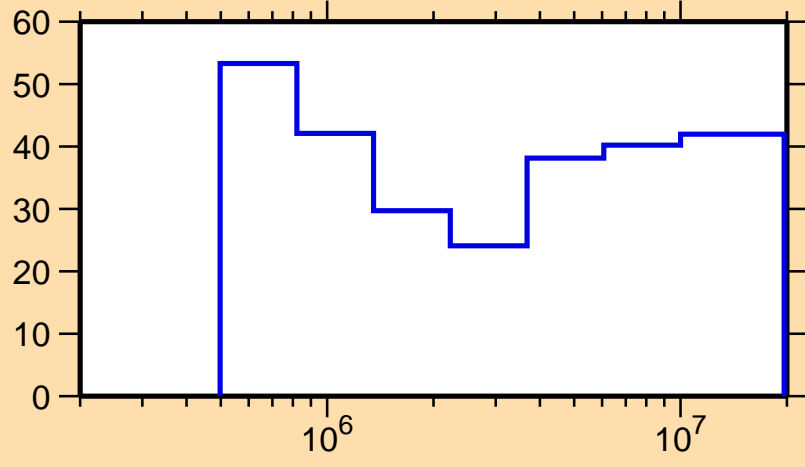
\Delta\sigma/\sigma vs. E for ^{156}\text{Ho}(n,n_1)
