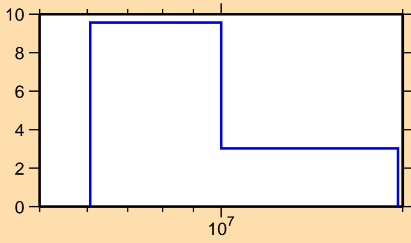
\Delta\sigma/\sigma vs. E for ^{156}\text{Ho}(n,\text{el.})
