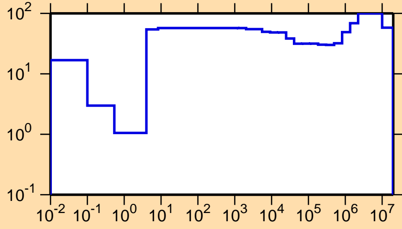
\Delta\sigma/\sigma vs. E for ^{156}\text{Ho}(n,\gamma)
