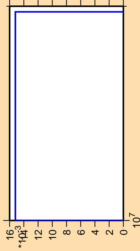
\Delta\sigma/\sigma vs. E for ^{156}\text{Ho}(n,3n\alpha)
