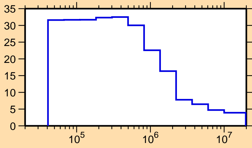
\Delta\sigma/\sigma vs. E for ^{156}\text{Ho}(n,\text{nonel.})
