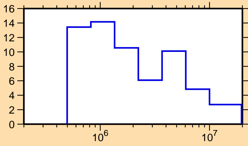
\Delta\sigma/\sigma vs. E for ^{156}\text{Ho}(n,\text{tot.})
