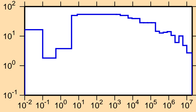
\Delta\sigma/\sigma vs. E for ^{156}\text{Ho}(n,\text{tot.})
