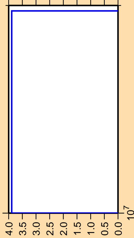
\Delta\sigma/\sigma vs. E for ^{156}\text{Ho} (mt 34)
