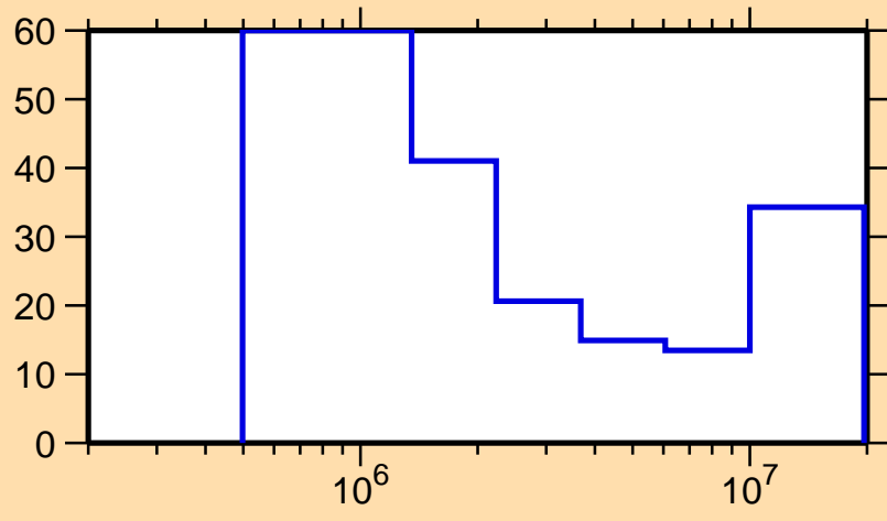
\Delta\sigma/\sigma vs. E for ^{156}\text{Ho}(n,n\text{cont.})
