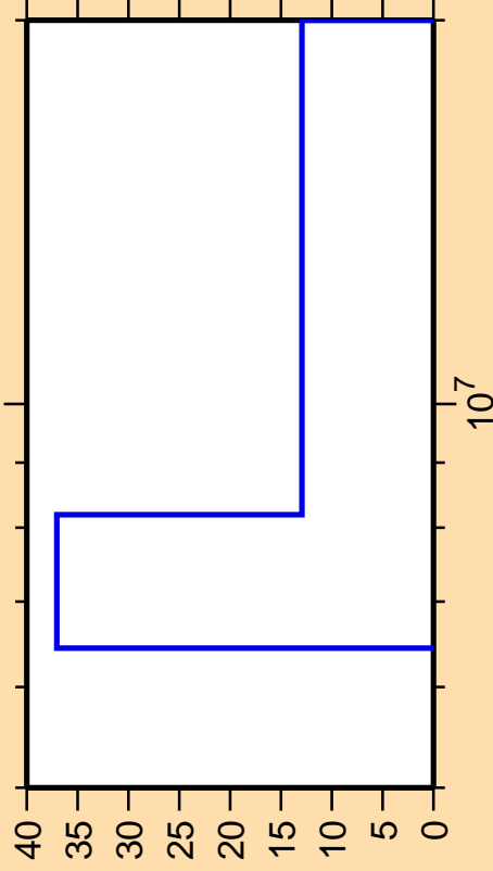
\Delta\sigma/\sigma vs. E for ^{156}\text{Ho}(n,2n)
