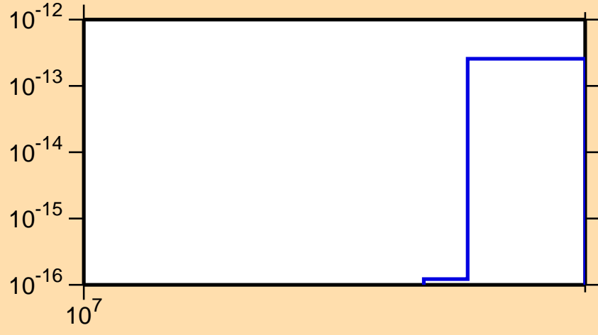
\sigma vs. E for ^{156}\text{Ho}(n,3n\alpha)
