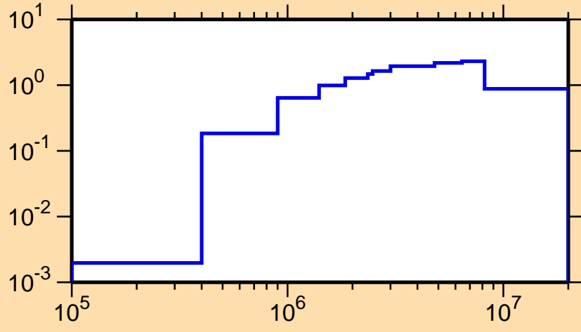
\sigma vs. E for ^{156}\text{Ho}(n,n\text{cont.})
