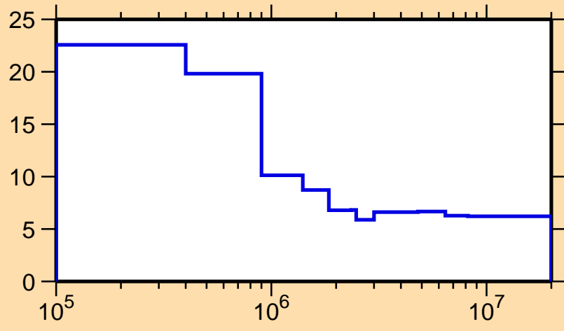
\Delta\sigma/\sigma vs. E for ^{156}\text{Ho}(n,n\text{onel.})
