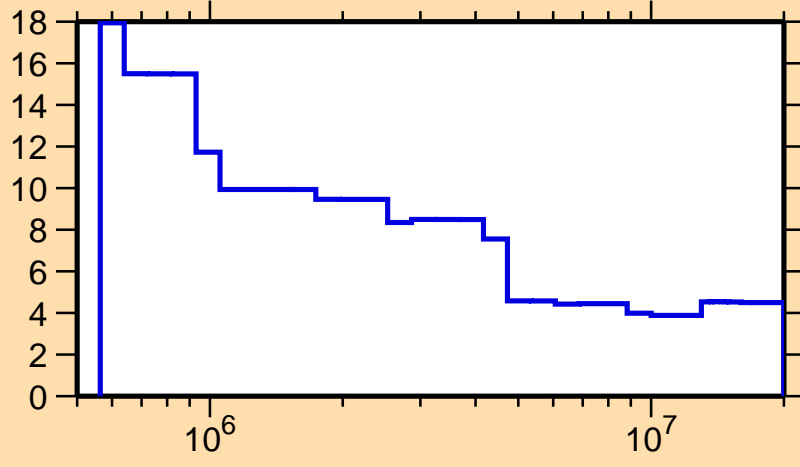
\Delta\sigma/\sigma vs. E for ^{157}\text{Ho}(n,n\text{onel.})
