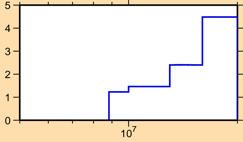
\Delta\sigma/\sigma vs. E for ^{157}\text{Ho}(n,\text{tot.})
