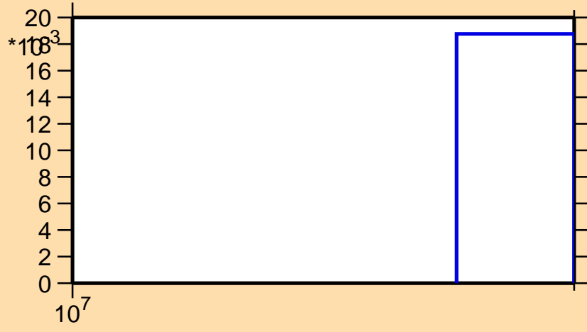
\sigma vs. E for ^{157}\text{Ho}(n,3n)
