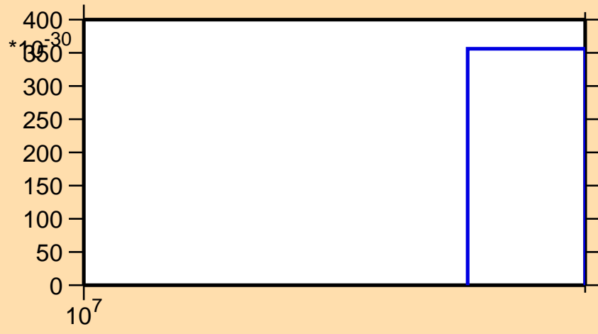
\sigma vs. E for ^{157}\text{Ho} (mt 42)
