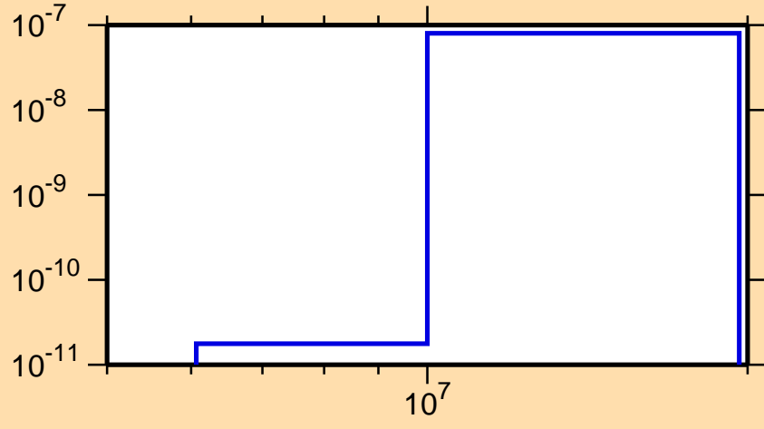
\sigma vs. E for ^{157}\text{Ho}(n,p\alpha)
