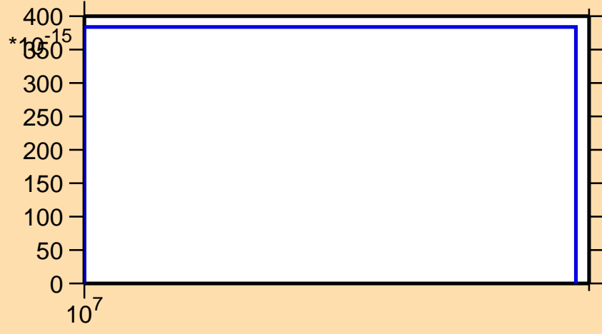
\sigma vs. E for ^{157}\text{Ho}(n,\text{pd})
