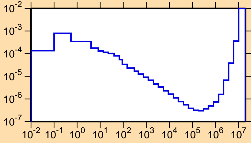
\sigma vs. E for ^{157}\text{Ho}(n,\alpha)
