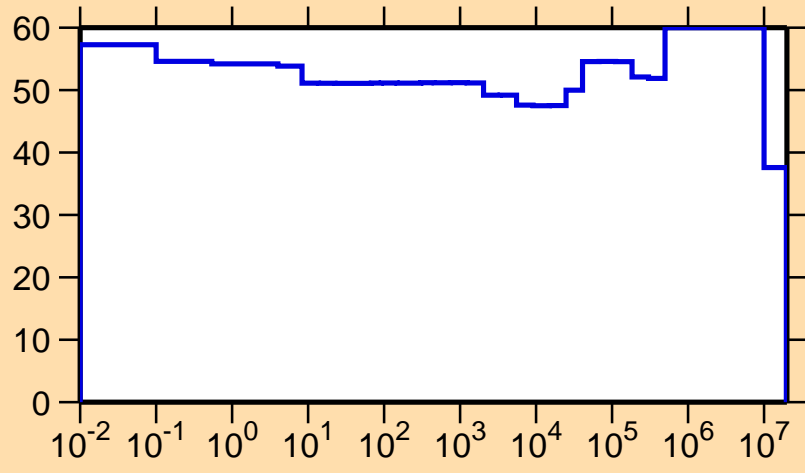
\Delta\sigma/\sigma vs. E for ^{157}\text{Ho}(n,p)
