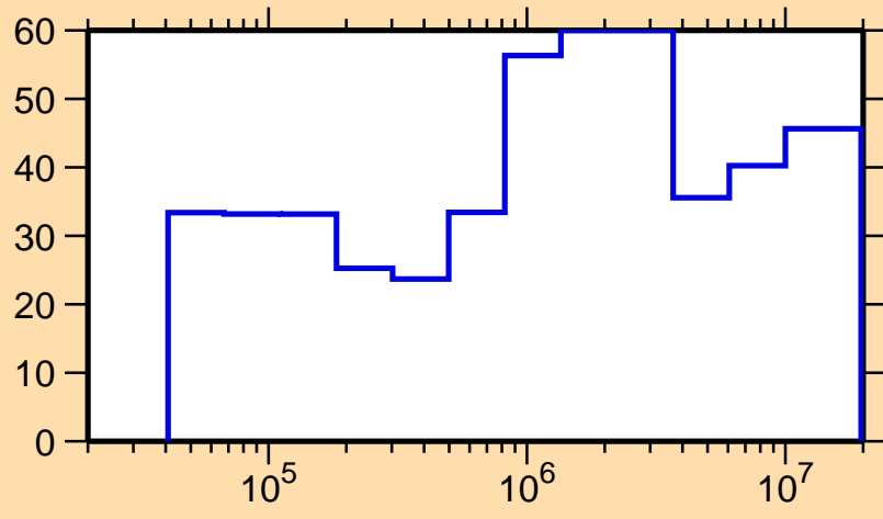
\Delta\sigma/\sigma vs. E for ^{157}\text{Ho}(n,n_1)
