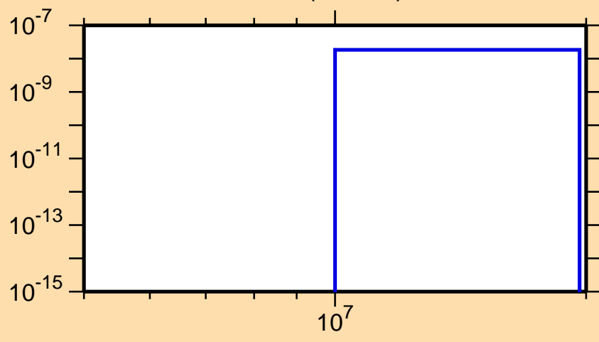
\sigma vs. E for ^{157}\text{Ho}(n,\text{He3})
