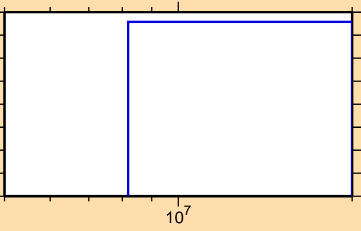
\sigma vs. E for ^{157}\text{Ho}(n,\text{He3})
