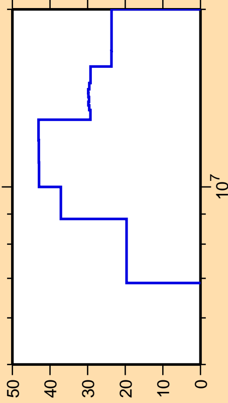
\Delta\sigma/\sigma vs. E for ^{158}\text{Ho}(n,n\text{cont.})
