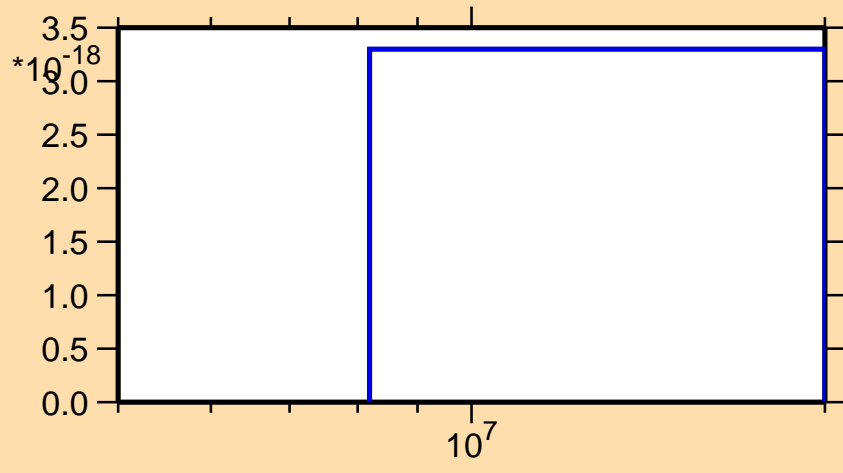
\sigma vs. E for ^{158}\text{Ho} (mt 11)
