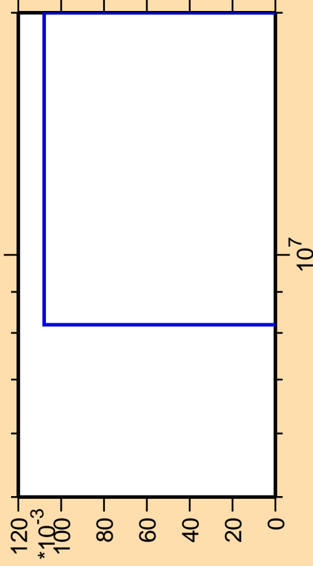
\Delta\sigma/\sigma vs. E for ^{158}\text{Ho}(n,pd)
