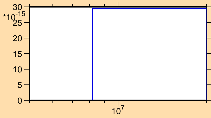
\sigma vs. E for ^{158}\text{Ho}(n,pd)
