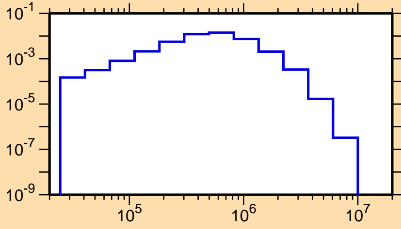
\sigma vs. E for ^{158}\text{Ho}(n,n_1)
