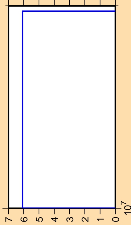
\Delta\sigma/\sigma vs. E for ^{158}\text{Ho} (mt 45)
