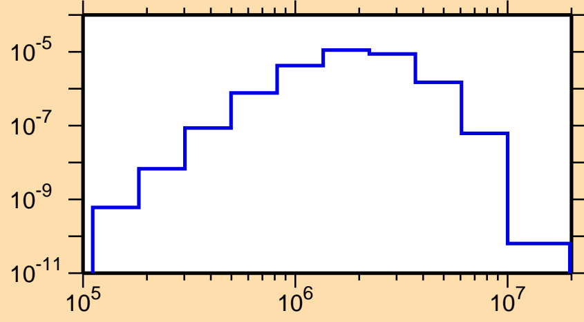
\sigma vs. E for ^{158}\text{Ho}(n,n_4)
