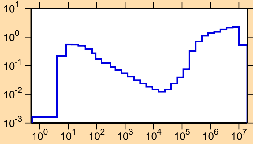
\sigma vs. E for ^{158}\text{Ho}(n,\text{inel.})
