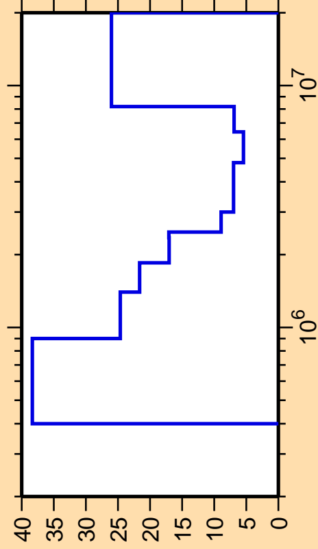
\Delta\sigma/\sigma vs. E for ^{158}\text{Ho}(n,\text{ncont.})
