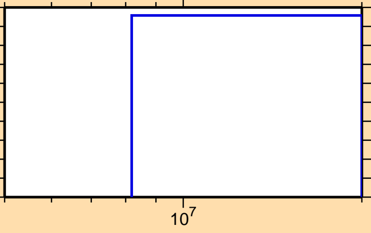
\sigma vs. E for ^{158}\text{Ho}(n,\text{pd})
