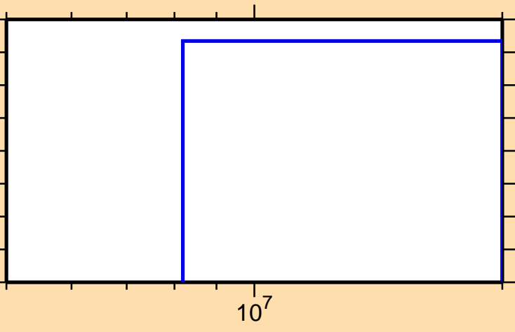
\sigma vs. E for ^{158}\text{Ho}(n,2np)
