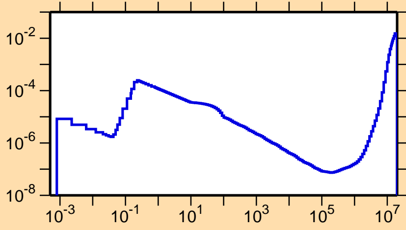
\sigma vs. E for ^{159}\text{Ho}(n,\alpha)
