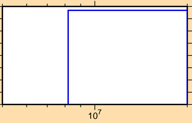
\sigma vs. E for ^{159}\text{Ho}(n,2n\alpha)
