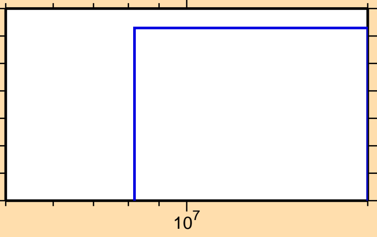
\sigma vs. E for ^{159}\text{Ho}(n,2n)
