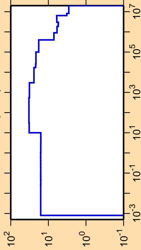
\Delta\sigma/\sigma vs. E for ^{159}\text{Ho}(n,\text{el.})
