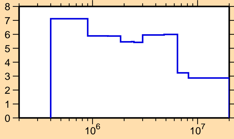
\Delta\sigma/\sigma vs. E for ^{159}\text{Ho}(n,\text{el.})
