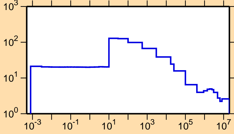
\sigma vs. E for ^{159}\text{Ho}(n,\text{el.})
