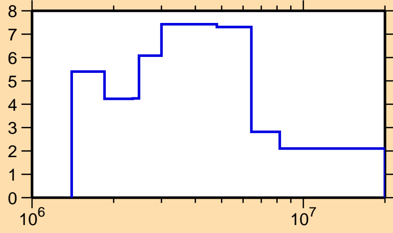
\Delta\sigma/\sigma vs. E for ^{160}\text{Ho}(n,\text{el.})
