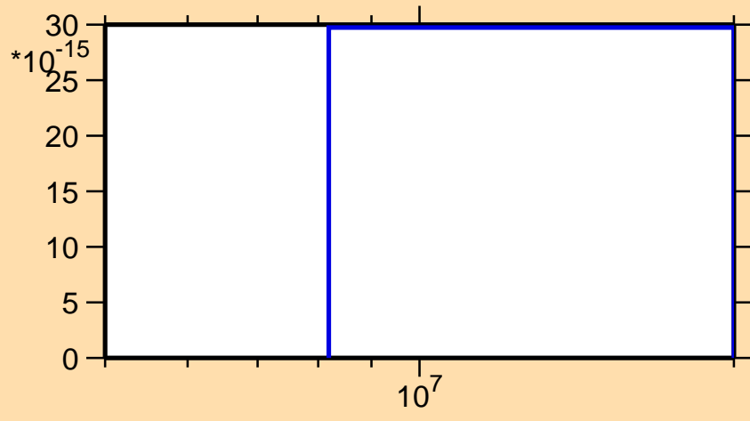
\sigma vs. E for ^{160}\text{Ho}(\text{mt117})
