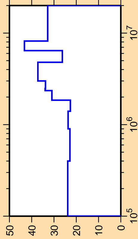
\Delta\sigma/\sigma vs. E for ^{160}\text{Ho}(n,n_4)
