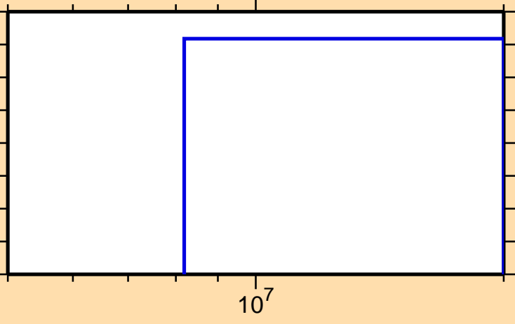
\sigma vs. E for ^{160}\text{Ho}(\text{mt117})
