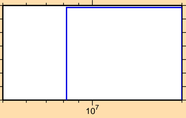
\sigma vs. E for ^{160}\text{Ho} (mt 11)
