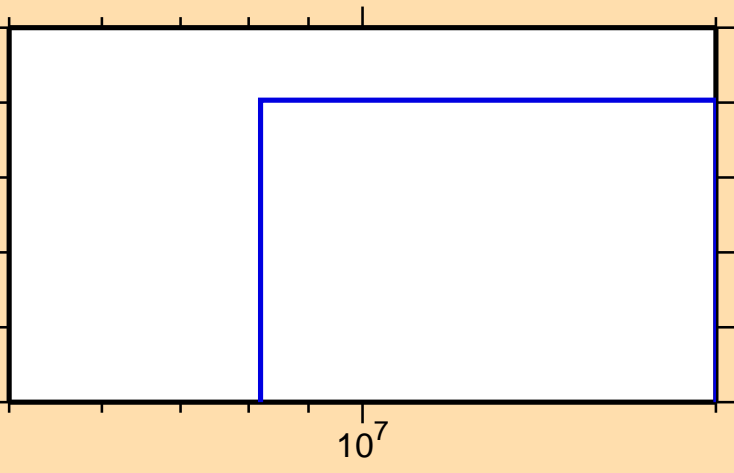
\sigma vs. E for ^{160}\text{Ho}(n,2np)
