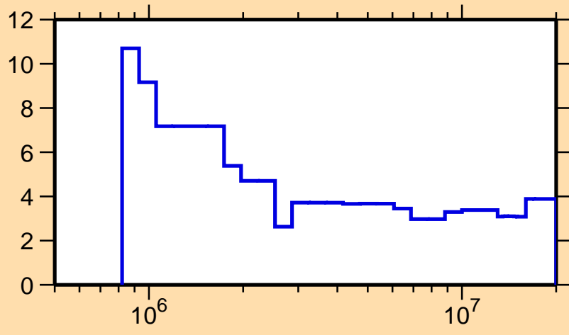
\Delta\sigma/\sigma vs. E for ^{160}\text{Ho}(n,n\text{onel.})
