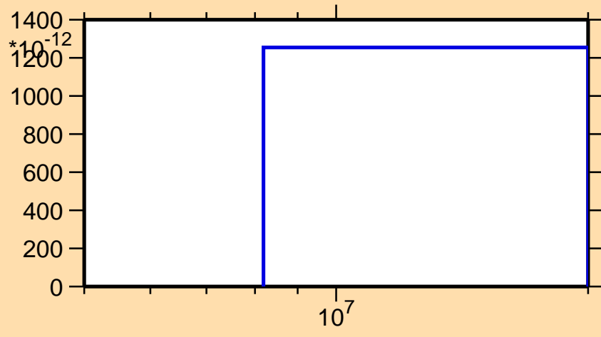
\sigma vs. E for ^{160}\text{Ho}(n,p\alpha)
