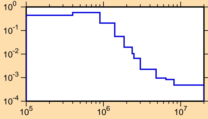
\sigma vs. E for ^{161}\text{Ho}(n,n_1)
