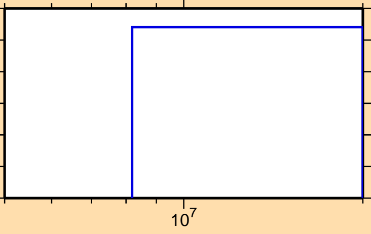
\sigma vs. E for ^{161}\text{Ho}(n,t)
