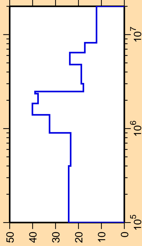
\Delta\sigma/\sigma vs. E for ^{161}\text{Ho}(n,n_1)
