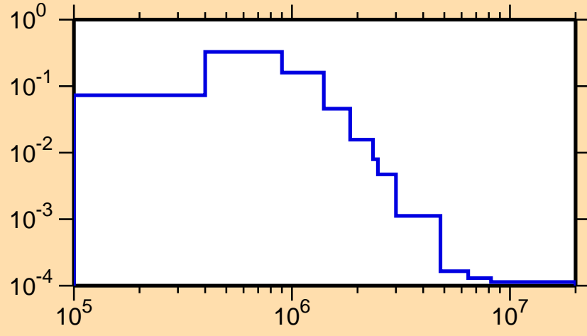
\sigma vs. E for ^{161}\text{Ho}(n,n_3)
