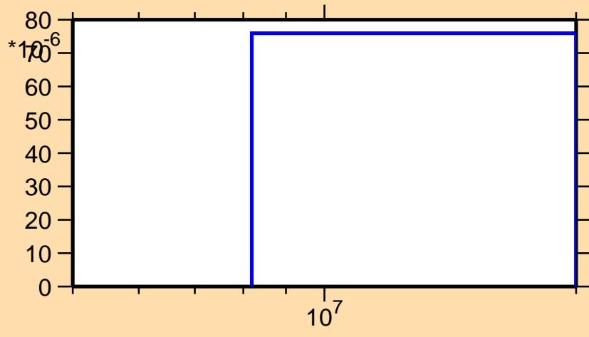
\sigma vs. E for ^{161}\text{Ho}(n,t)
