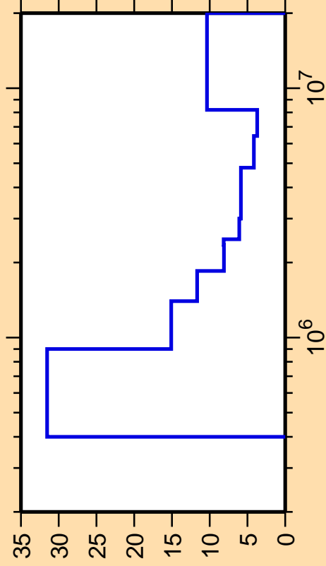
\Delta\sigma/\sigma vs. E for ^{161}\text{Ho}(n,n\text{cont.})
