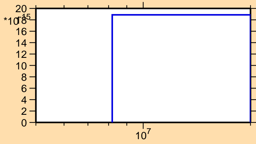
\sigma vs. E for ^{161}\text{Ho}(\text{mt117})
