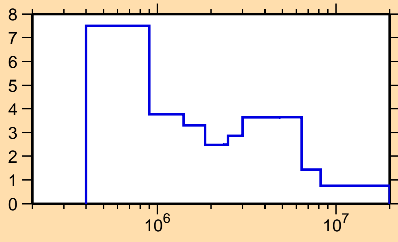
\Delta\sigma/\sigma vs. E for ^{161}\text{Ho}(n,\text{tot.})
