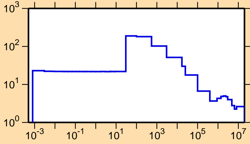
\sigma vs. E for ^{161}\text{Ho}(n,\text{el.})
