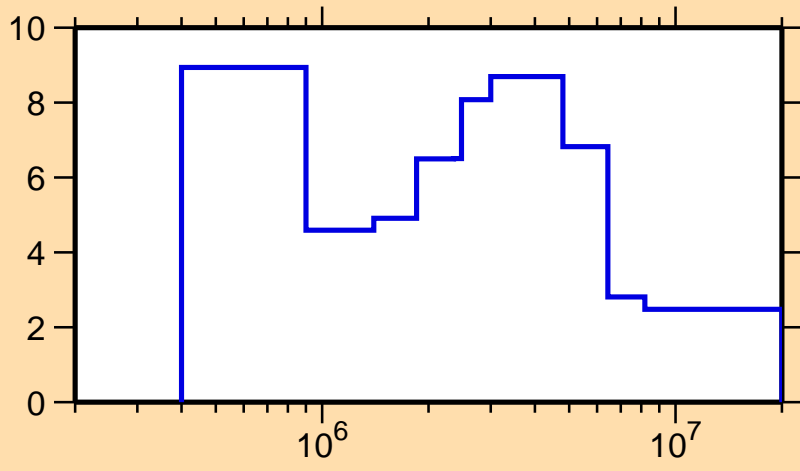
\Delta\sigma/\sigma vs. E for ^{161}\text{Ho}(n, el.)
