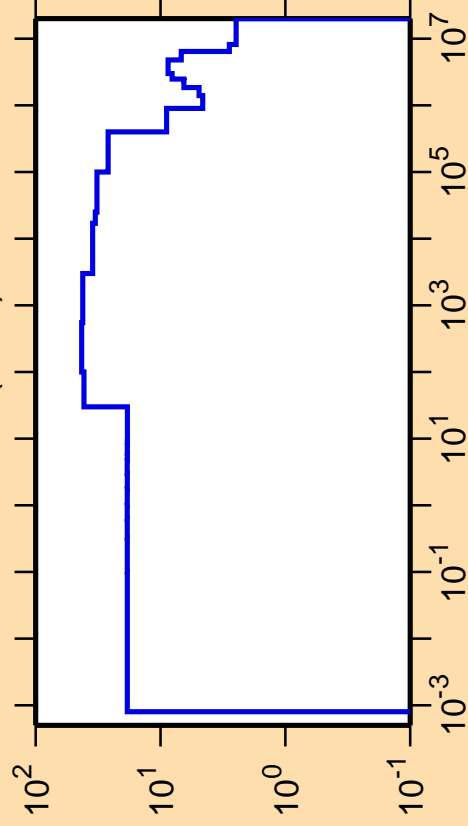
\Delta\sigma/\sigma vs. E for ^{161}\text{Ho}(n,\text{el.})
