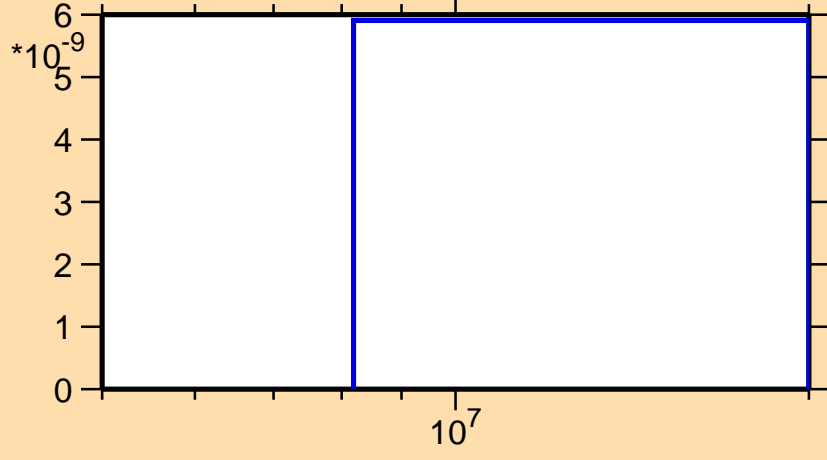
\sigma vs. E for ^{161}\text{Ho}(n,nt)
