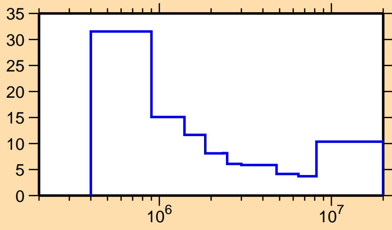
\Delta\sigma/\sigma vs. E for ^{161}\text{Ho}(n,n\text{cont.})
