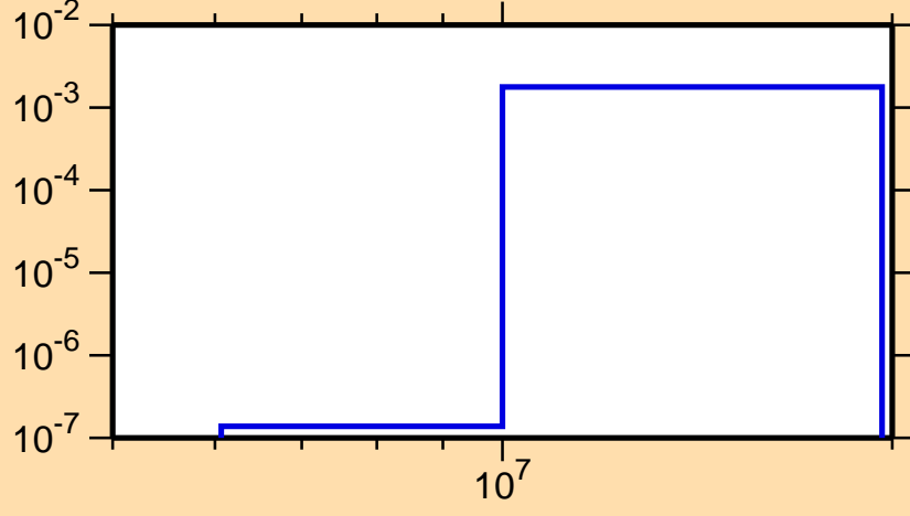
\sigma vs. E for ^{162}\text{Ho}(n,d)
