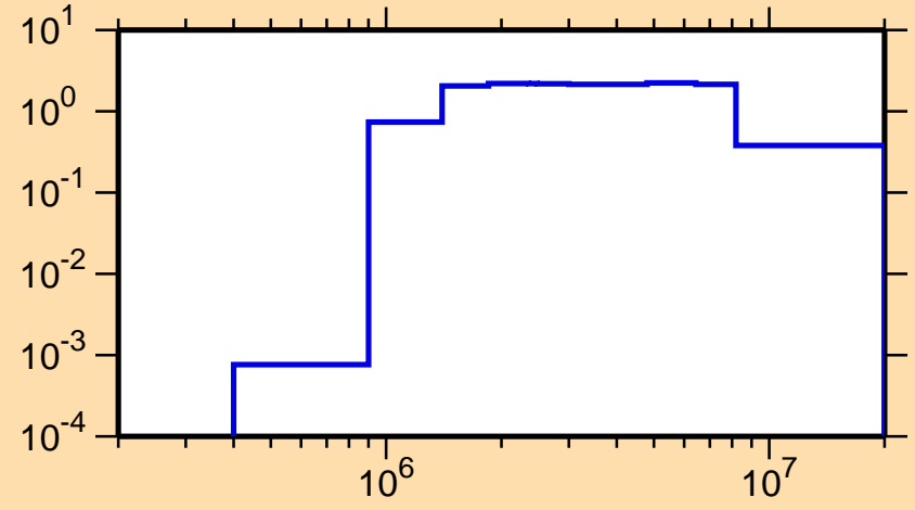
\sigma vs. E for ^{162}\text{Ho}(n,n\text{cont.})
