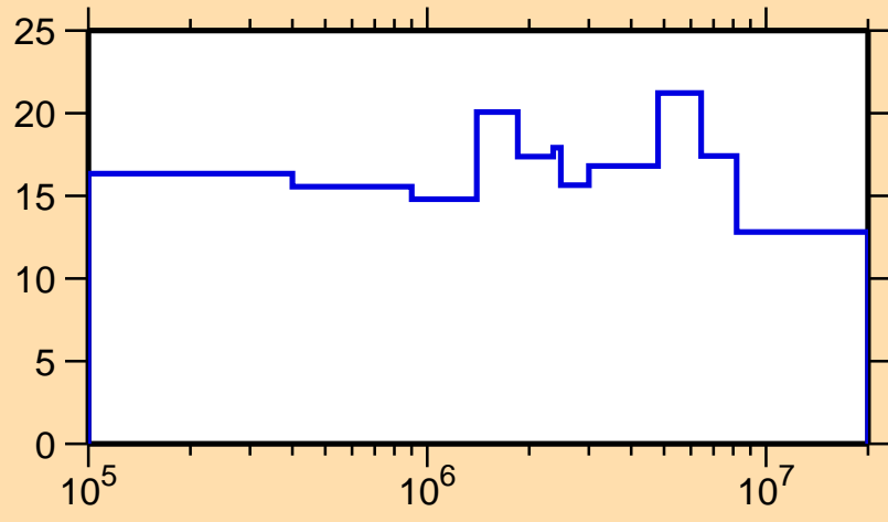
\Delta\sigma/\sigma vs. E for ^{162}\text{Ho}(n, n_1)
