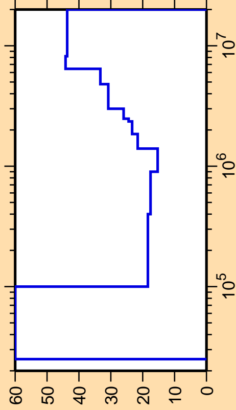
\Delta\sigma/\sigma vs. E for ^{162}\text{Ho}(n,n_2)
