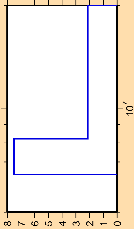
\Delta\sigma/\sigma vs. E for ^{162}\text{Ho}(n,2n)
