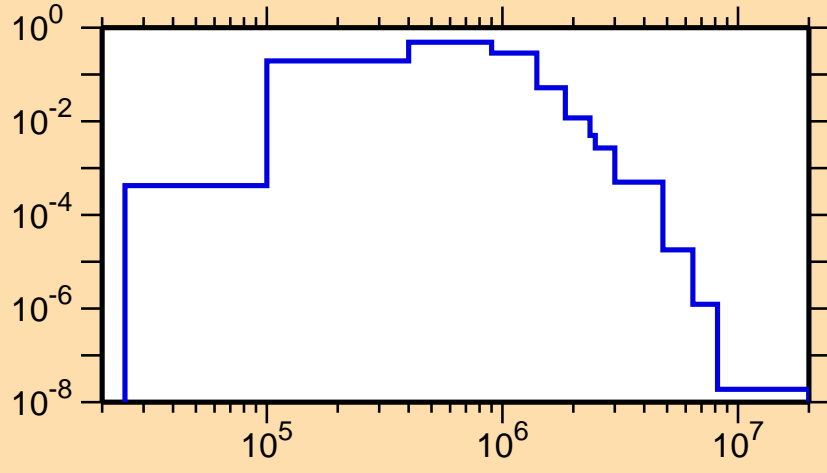
\sigma vs. E for ^{162}\text{Ho}(n,n_2)
