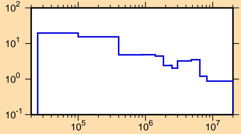
\Delta\sigma/\sigma vs. E for ^{162}\text{Ho}(n,\text{tot.})
