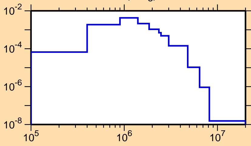
\sigma vs. E for ^{162}\text{Ho}(n,n_3)
