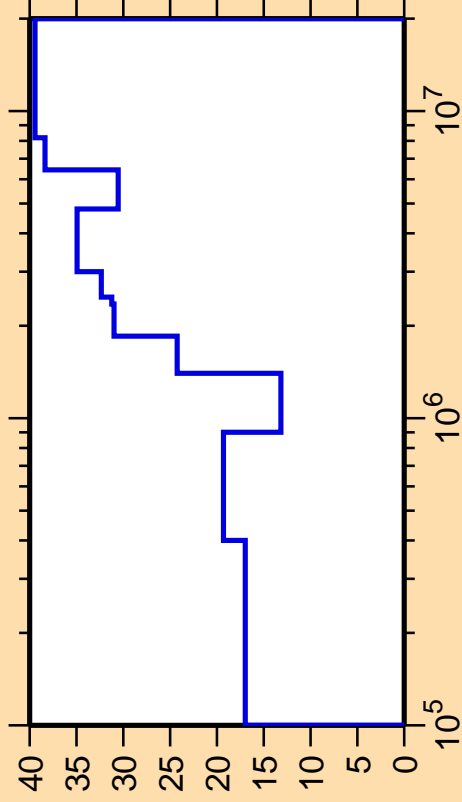
\Delta\sigma/\sigma vs. E for ^{162}\text{Ho}(n,n_3)
