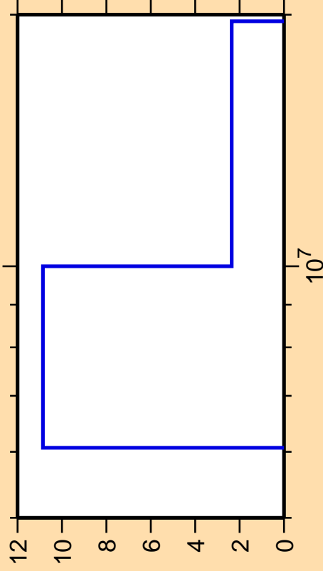
\Delta\sigma/\sigma vs. E for ^{162}\text{Ho}(n,2n)
