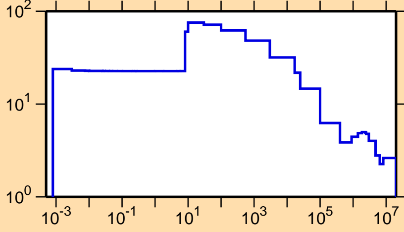
\sigma vs. E for ^{162}\text{Ho}(n,\text{el.})
