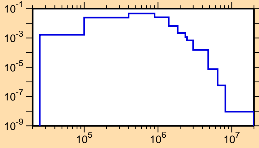
\sigma vs. E for ^{162}\text{Ho}(n,n_4)
