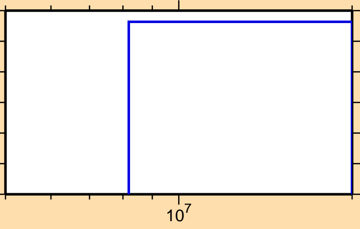
\sigma vs. E for ^{163}\text{Ho}(n,\text{He3})
