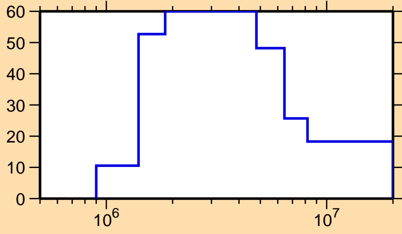
\Delta\sigma/\sigma vs. E for ^{163}\text{Ho}(n,p)
