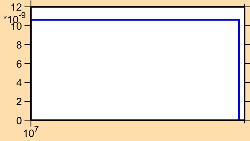
\sigma vs. E for ^{163}\text{Ho}(n,2np)
