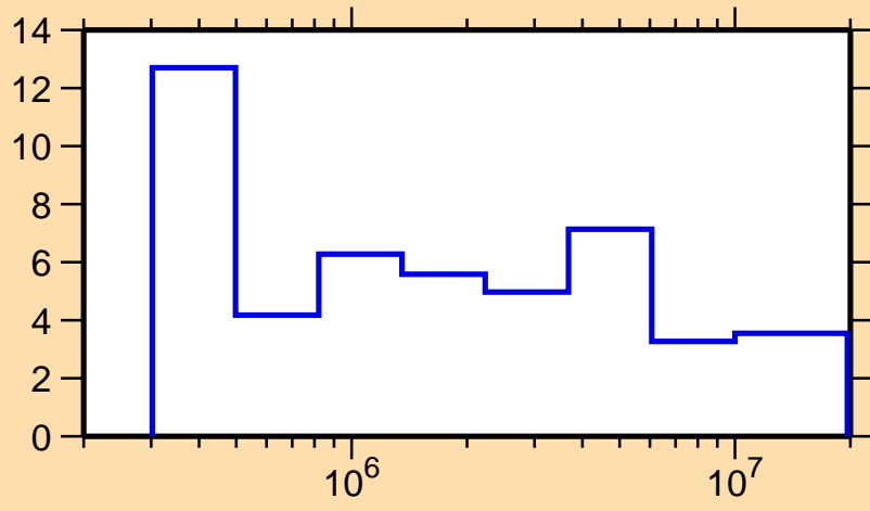
\Delta\sigma/\sigma vs. E for ^{163}\text{Ho}(n,\text{el.})
