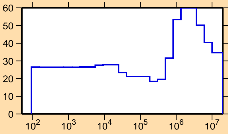
\Delta\sigma/\sigma vs. E for ^{163}\text{Ho}(n,n_1)
