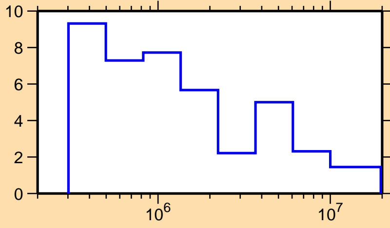
\Delta\sigma/\sigma vs. E for ^{163}\text{Ho}(n,\text{tot.})
