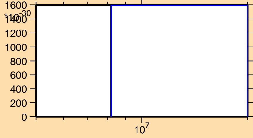
\sigma vs. E for ^{163}\text{Ho} (mt 42)
