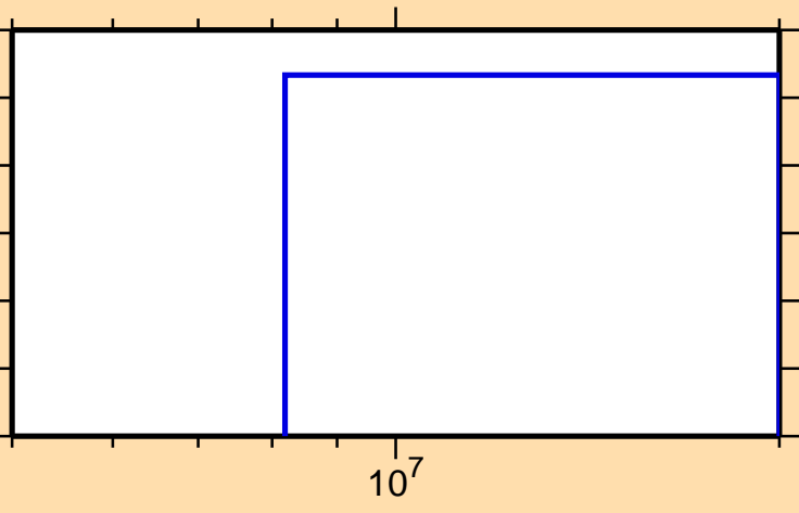
\sigma vs. E for ^{163}\text{Ho}(n,t)
