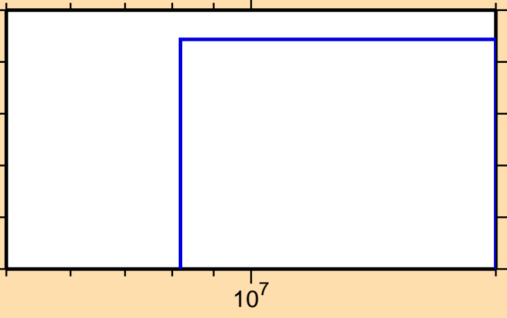
\sigma vs. E for ^{163}\text{Ho}(n,nt)
