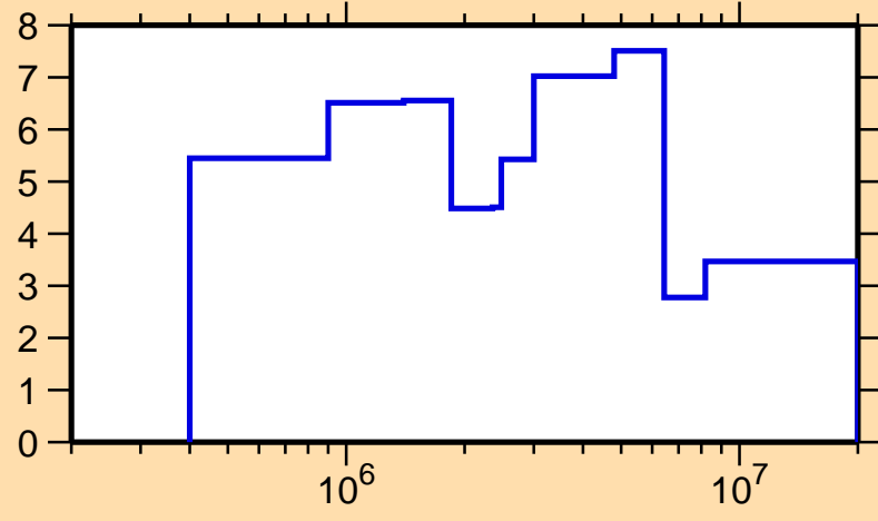
\Delta\sigma/\sigma vs. E for ^{163}\text{Ho}(n, el.)
