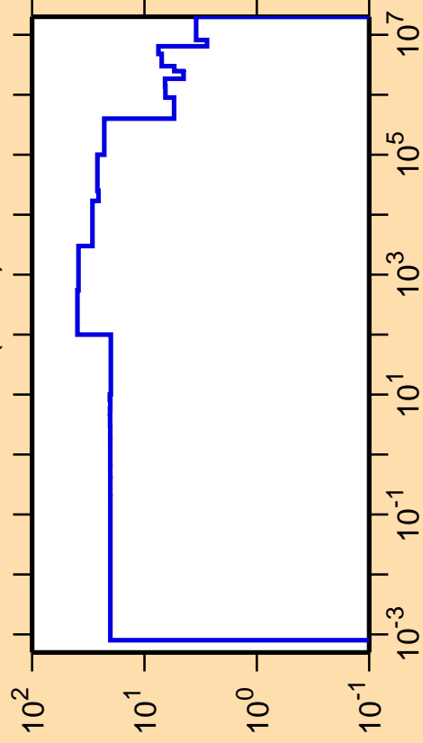
\Delta\sigma/\sigma vs. E for ^{163}\text{Ho}(n,\text{el.})
