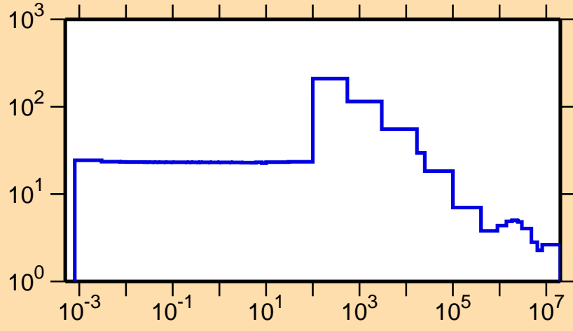
\sigma vs. E for ^{163}\text{Ho}(n,\text{el.})
